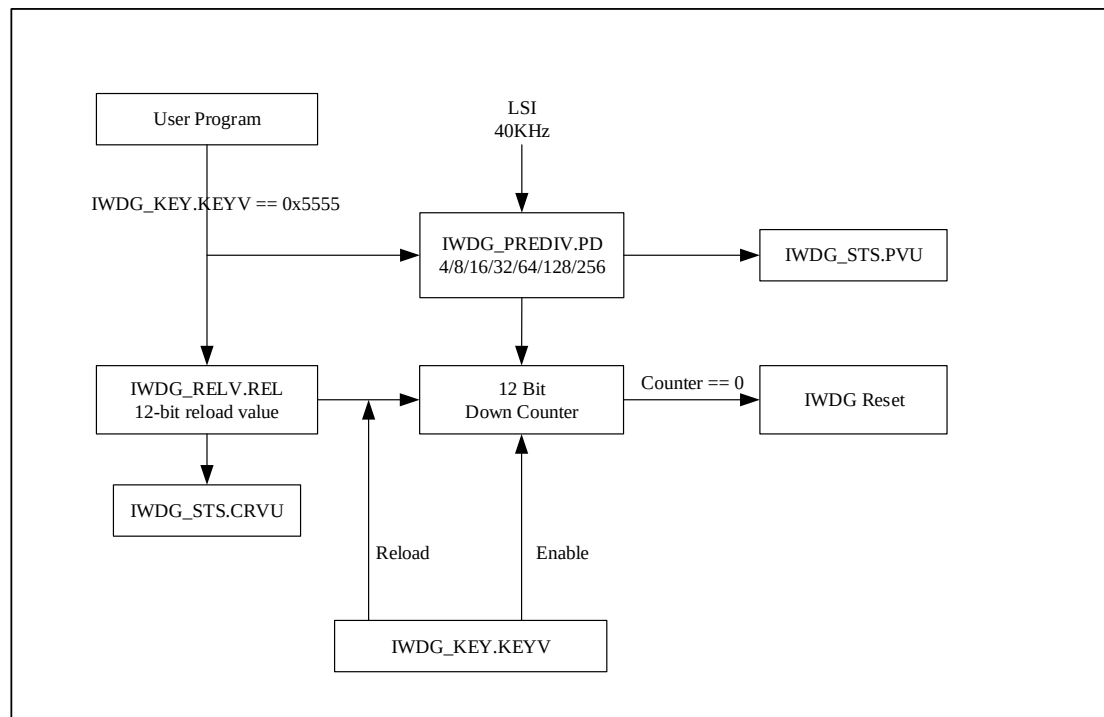
Figure 17-1 Functional block diagram of the independent watchdog module
