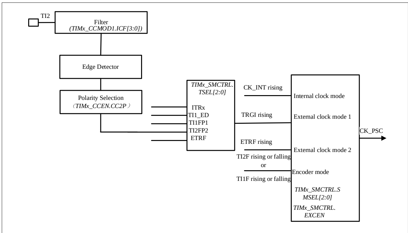
Figure 12-12 TI2 external clock connection example
