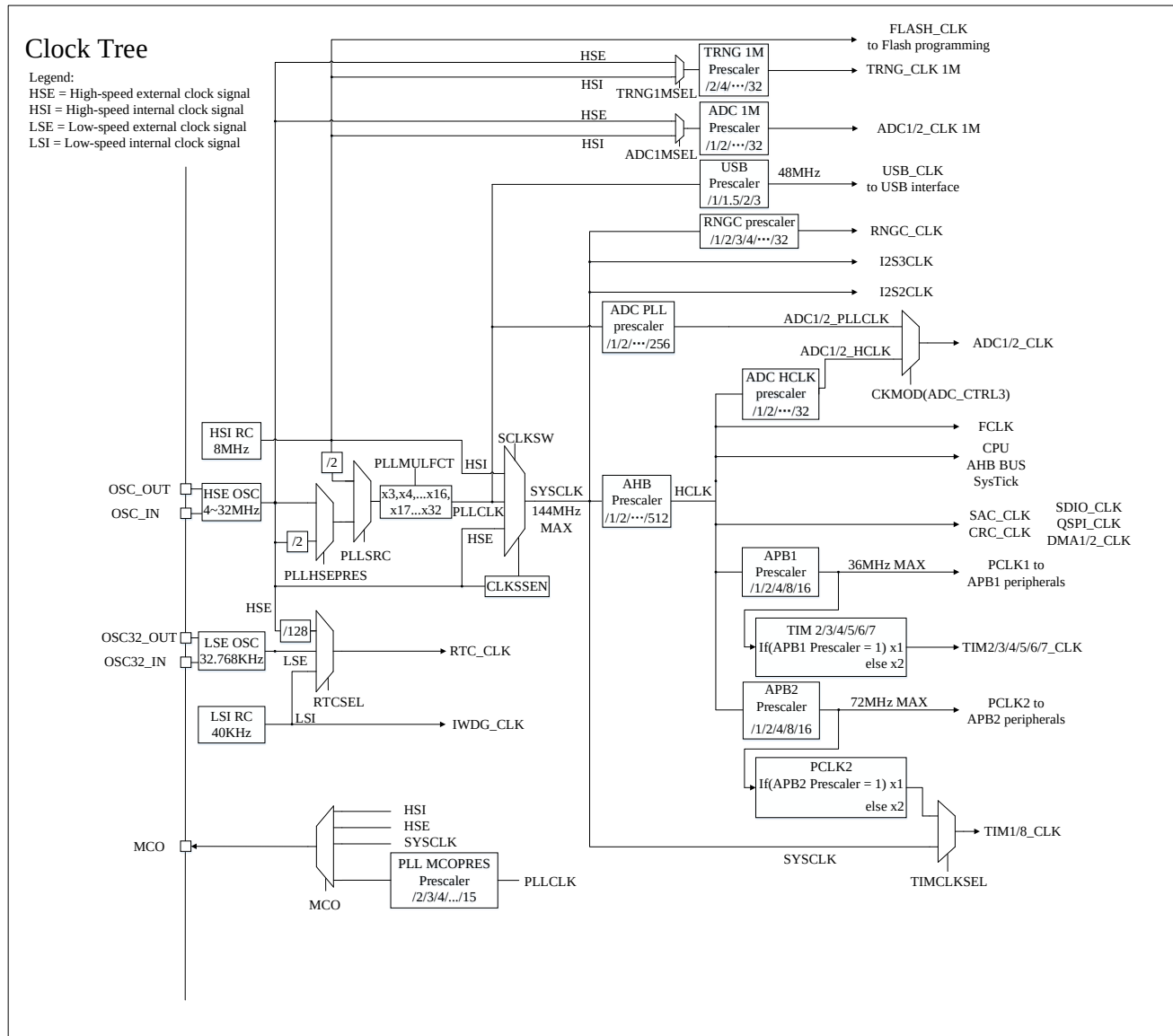
Figure 5-2 Clock Tree
