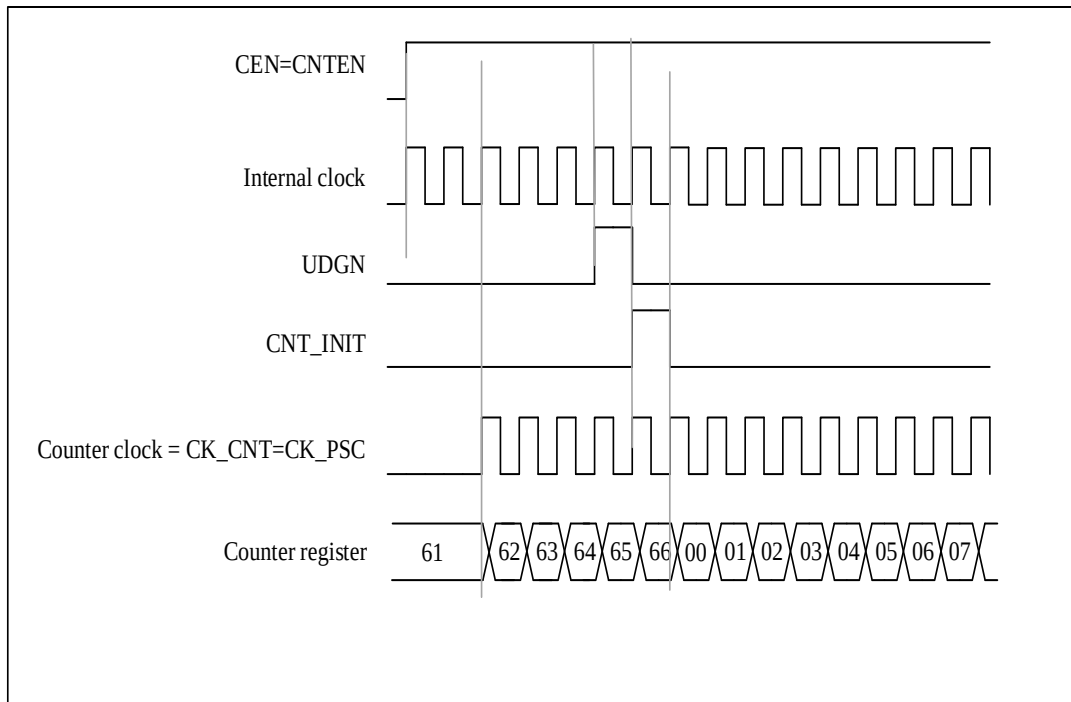
Figure 14-5 Control circuit in normal mode, internal clock divided by 1
