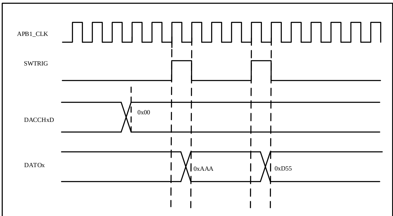
Figure 11-6 DAC conversion with LFSR waveform generation (enable software trigger)
