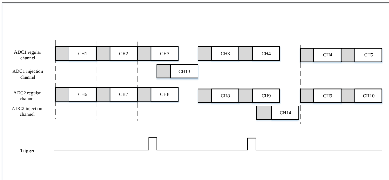
Figure 10-14 Combination of rotation mode and synchronous regular mode
