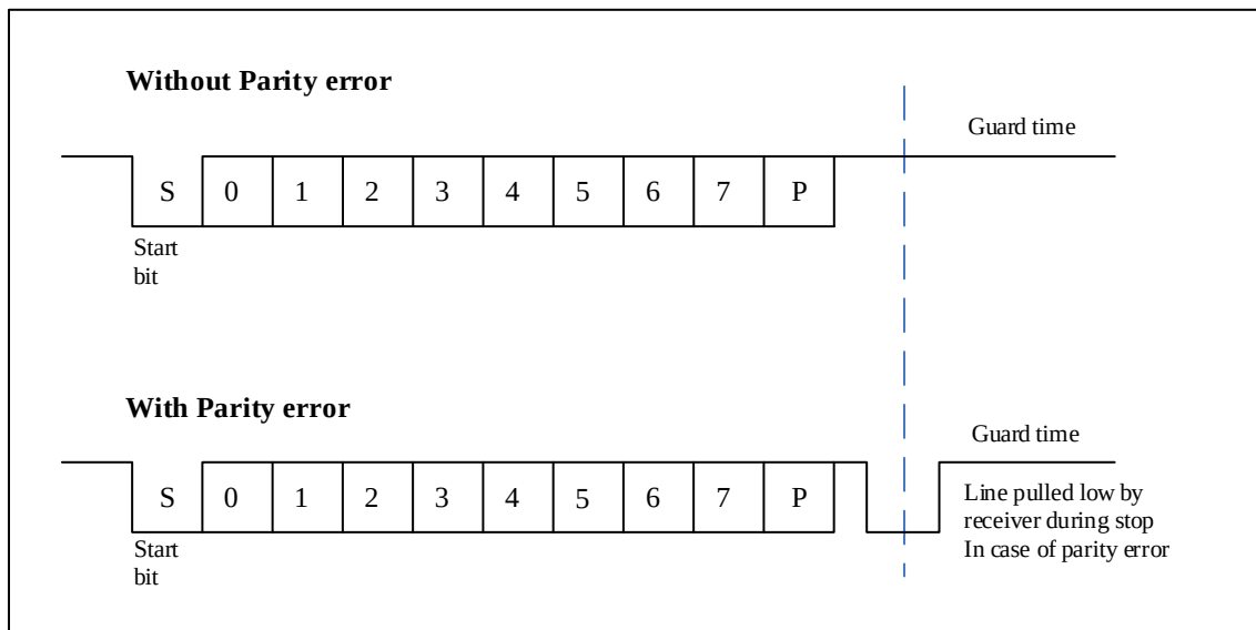
Figure 24-23 ISO7816-3 Asynchronous Protocol
