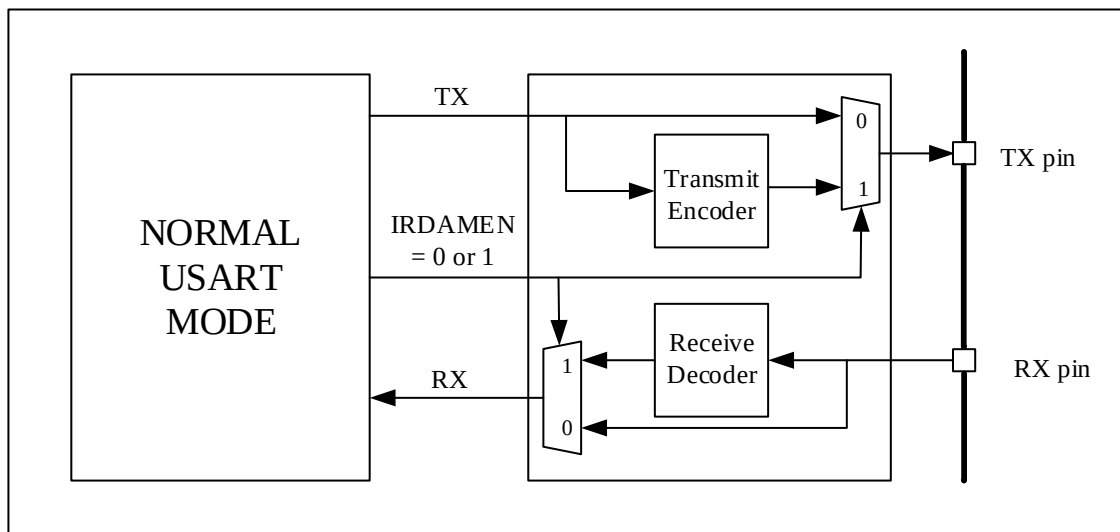
Figure 24-20 IrDA data Modulation (3/16)-normal mode
