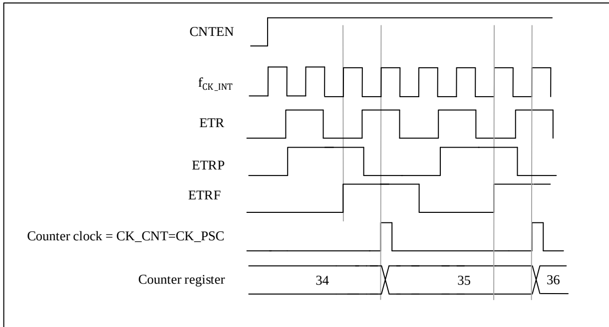
Figure 13-12 Control circuit in external clock mode 2
