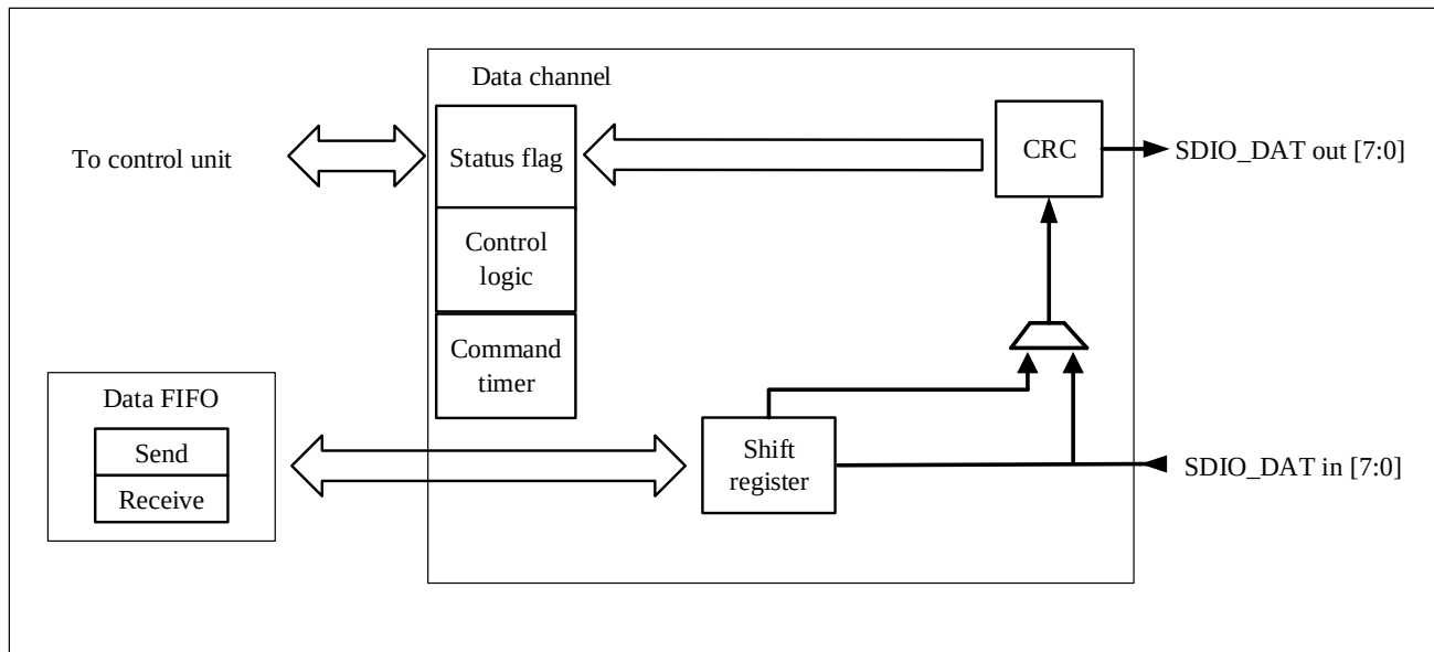
Figure 19-12 Data Channel
