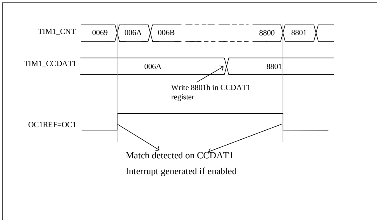
Figure 12-21 Output compare mode, toggle on OC1
