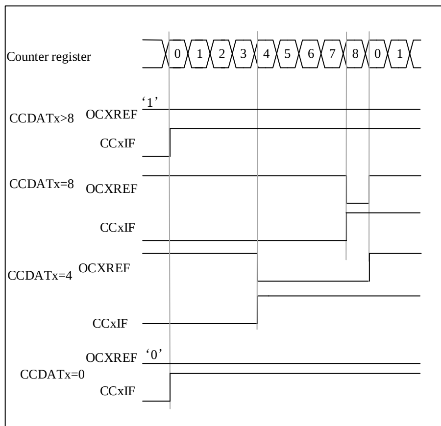
Figure 12-23 Edge-aligned PWM waveform (APR=8)
