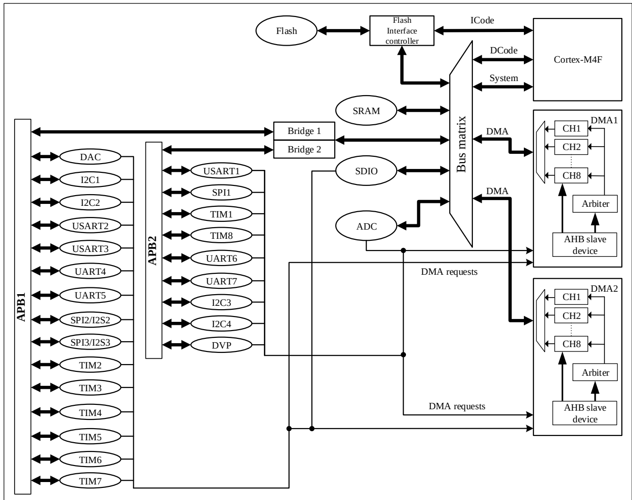
Figure 9-1 DMA block diagram
