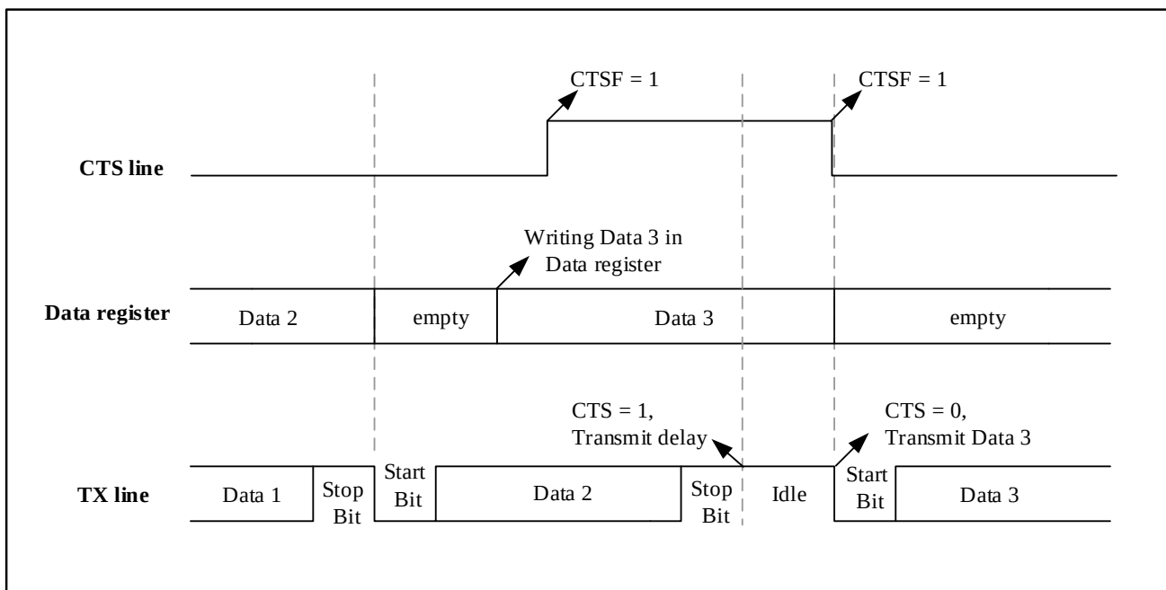
Figure 24-12 CTS flow controls
