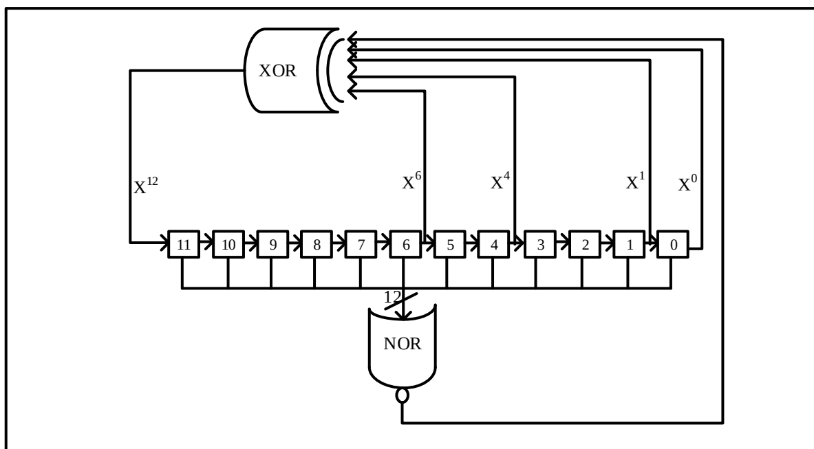
Figure 11-5 LFSR algorithm for DAC
