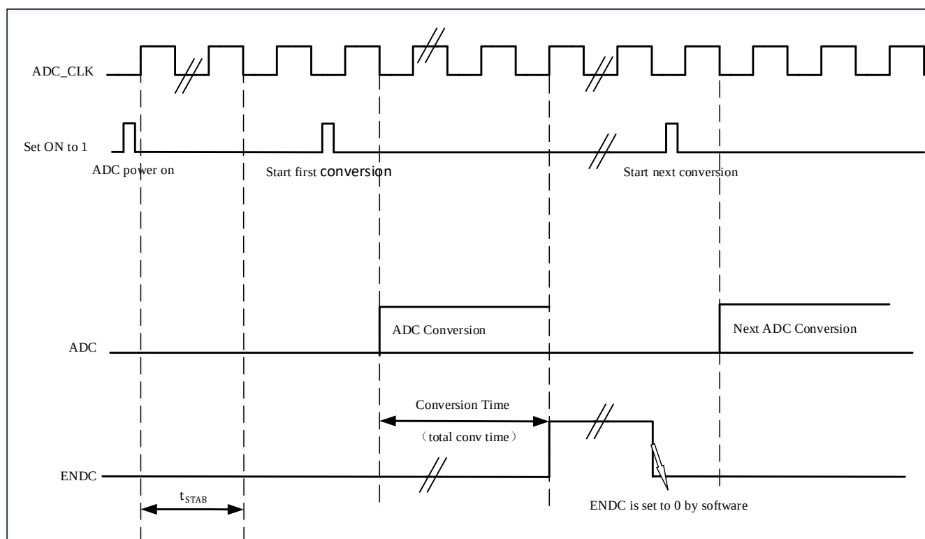
Figure 10-4 Timing diagram
