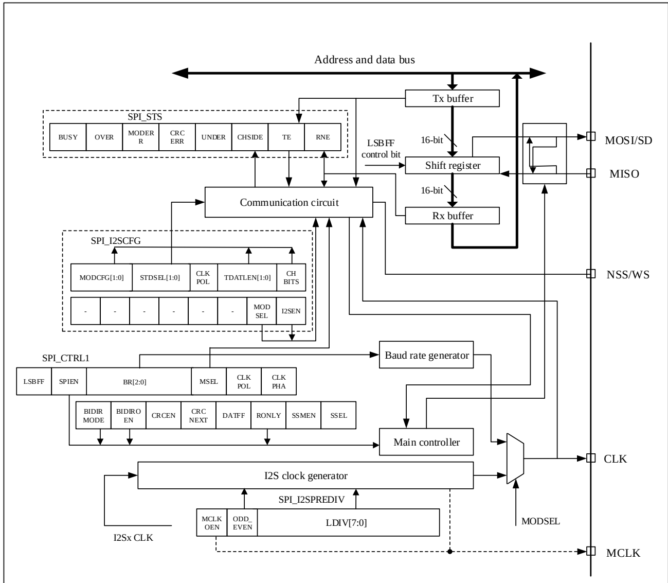
Figure 22-13 I 2 S block diagram
