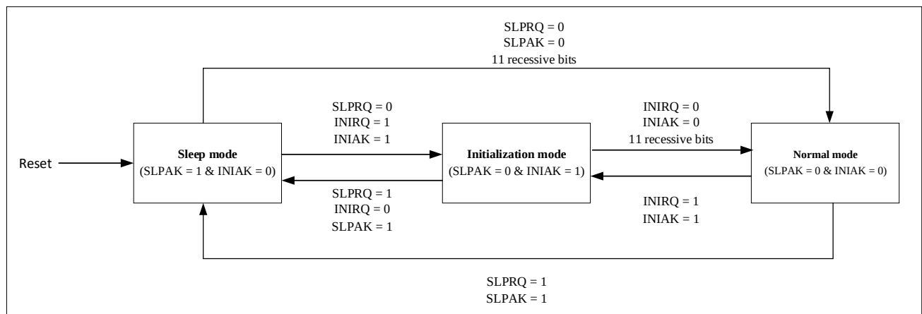
Figure 21-2 CAN working mode
