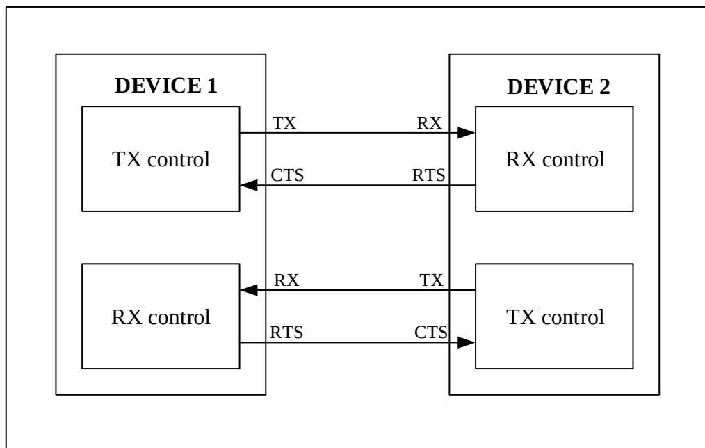
Figure 24-10 hardware flow control between two USART
