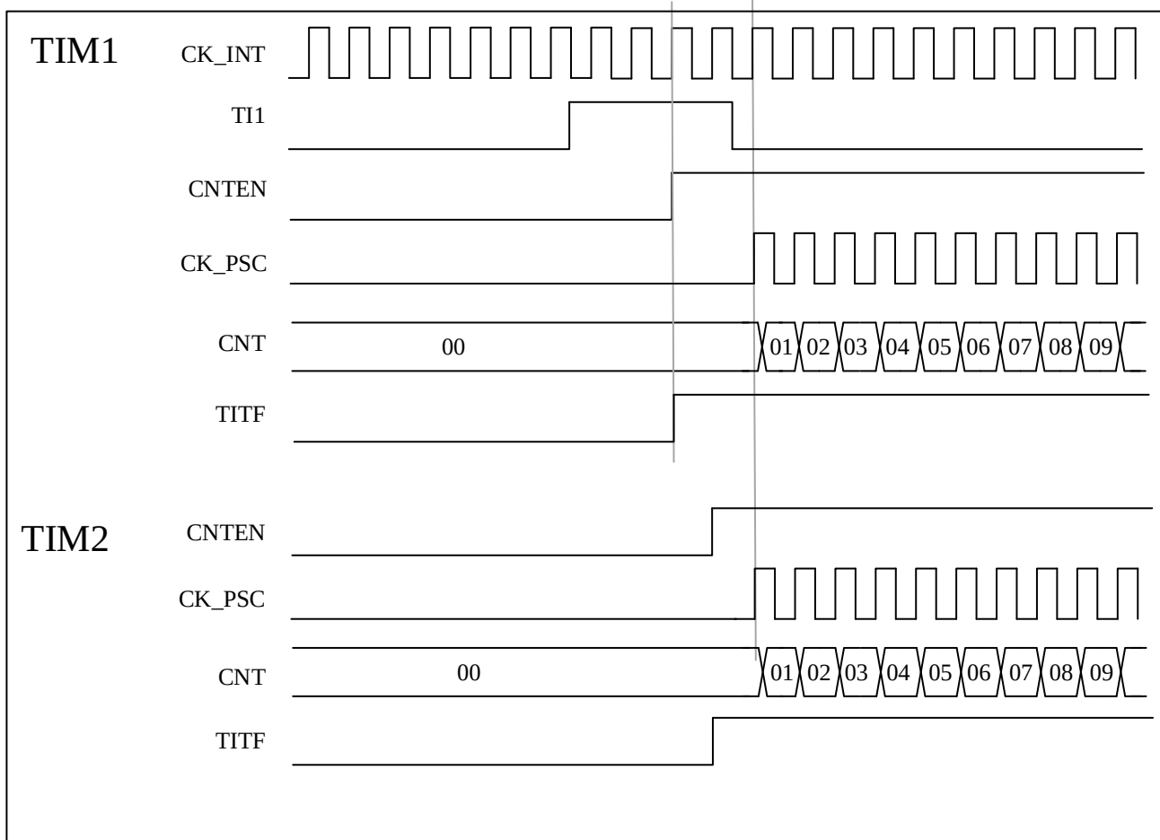
Figure 13-26 Triggers timers 1 and 2 using the TI1 input of TIM1
