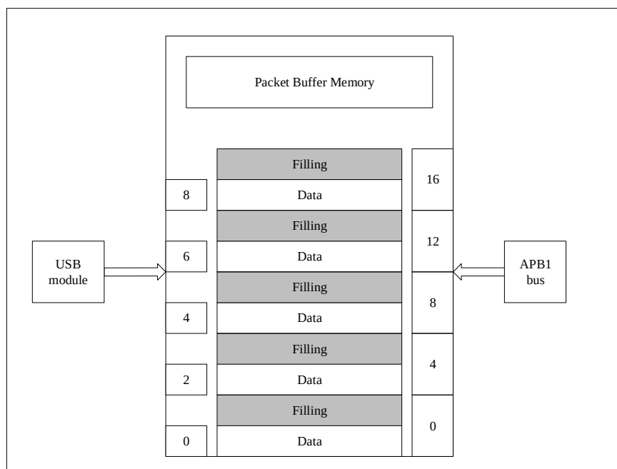
Figure 20-2 The user applications on the microcontrollers and the USB modules access Packet Buffer Memory
