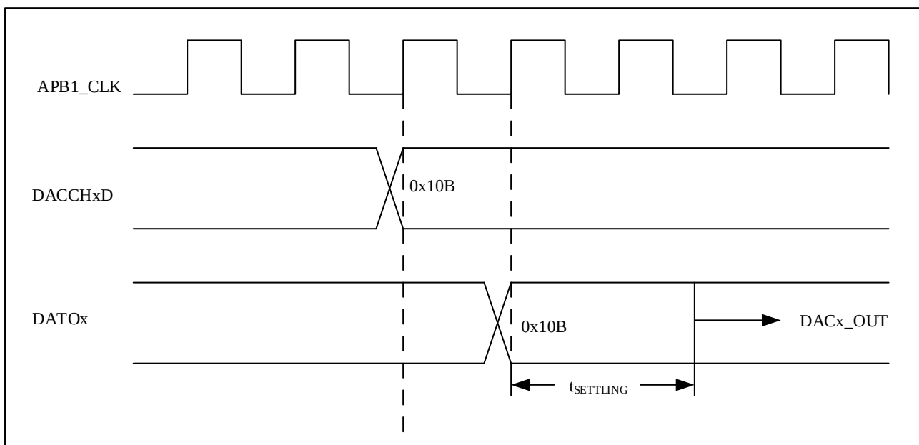
Figure 11-4 Time diagram of transitions with trigger disabled
