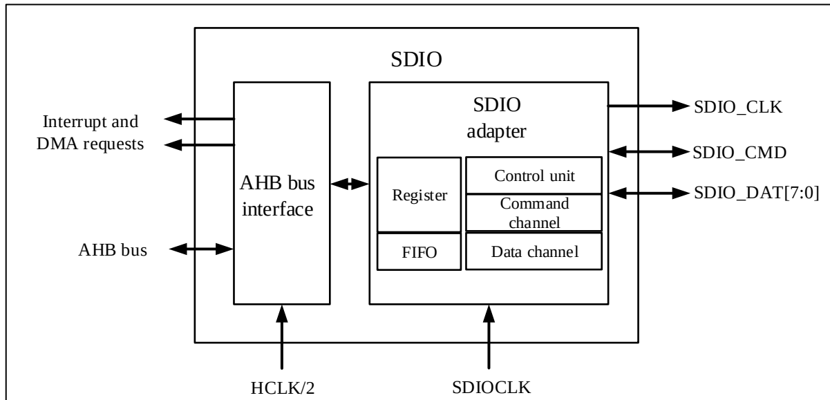
Figure 19-6 SDIO block diagram
