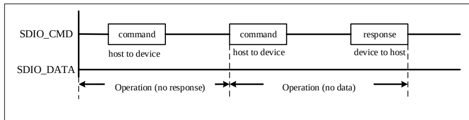
Figure 19-2 SDIO (multi) data block read operation
