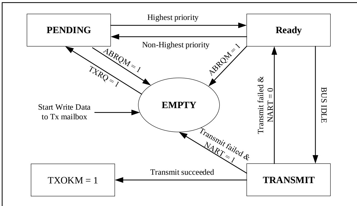
Figure 21-7 Send mailbox status
