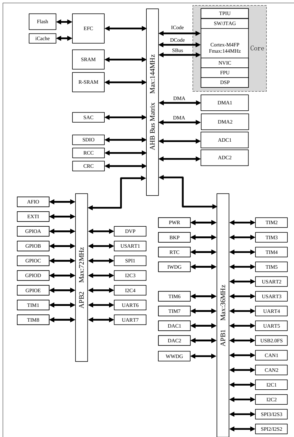
Figure 2-2 Bus architecture
