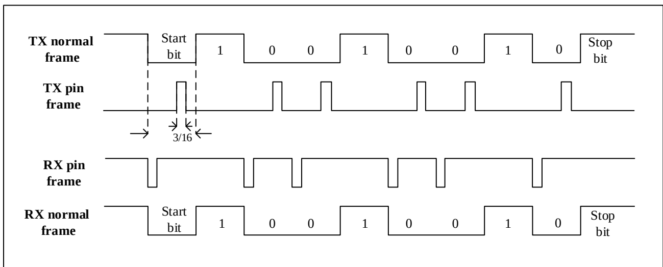
Figure 24-20 IrDA data Modulation (3/16)-normal mode
