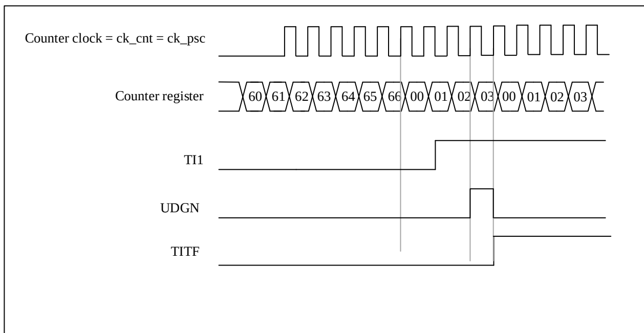
Figure 12-27 Control circuit in reset mode
