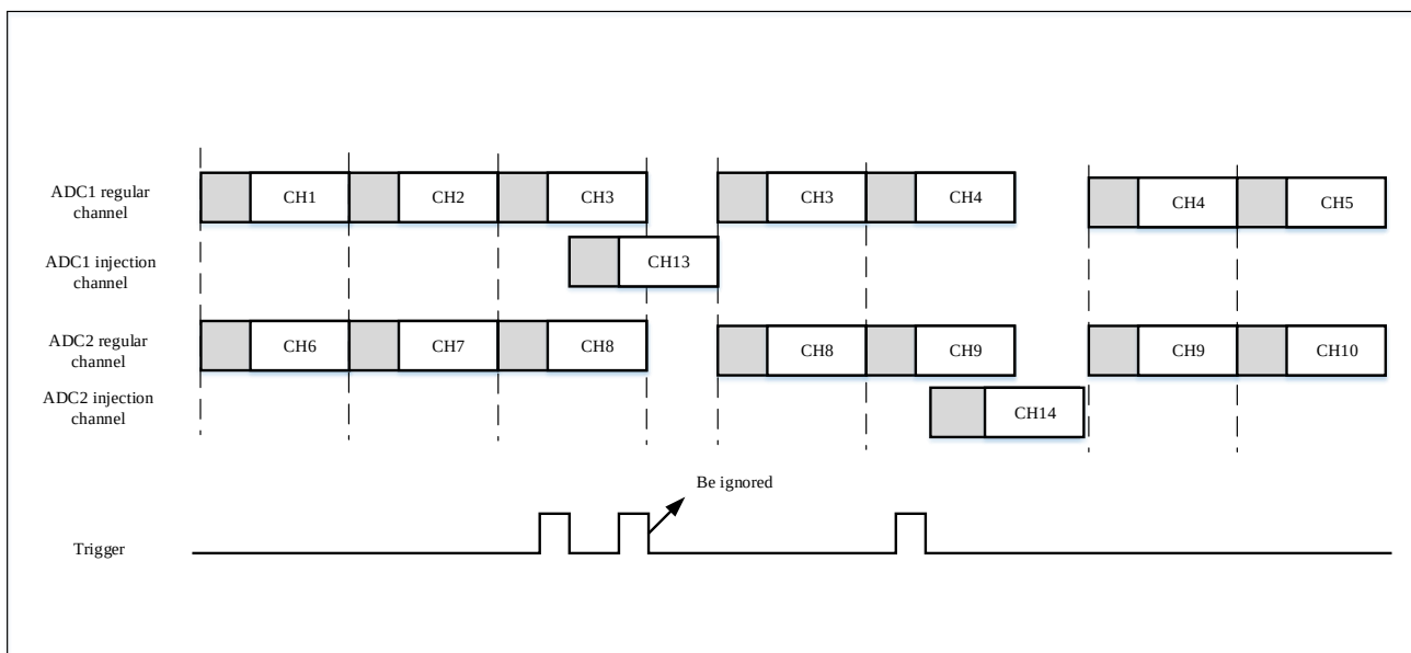
Figure 10-15 Injection trigger occurs during injection transition
