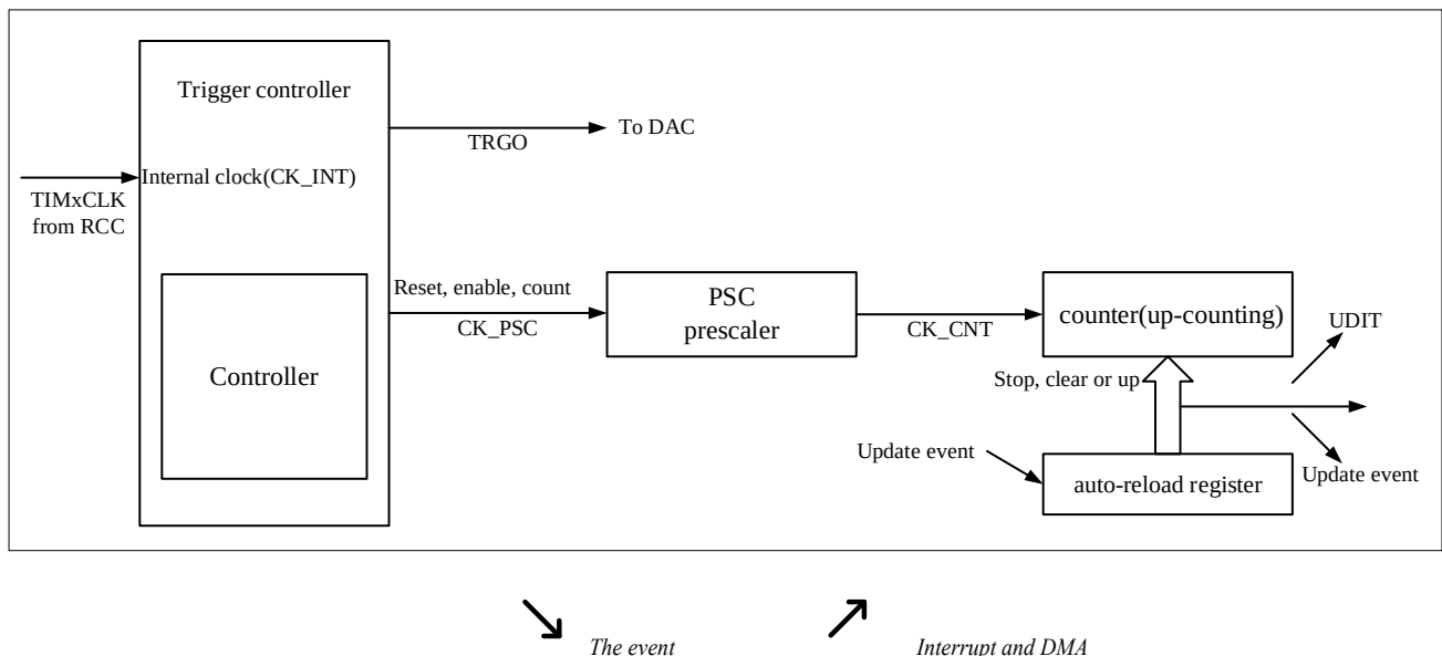
Figure 14-1 Block diagram of TIMx (x = 6 and 7)
