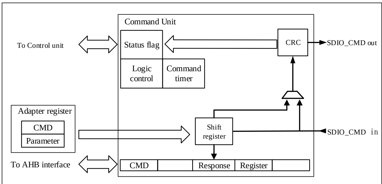
Figure 19-9 SDIO adapter command unit
