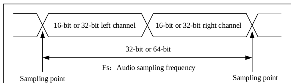
Figure 22-26 Audio sampling frequency definition
