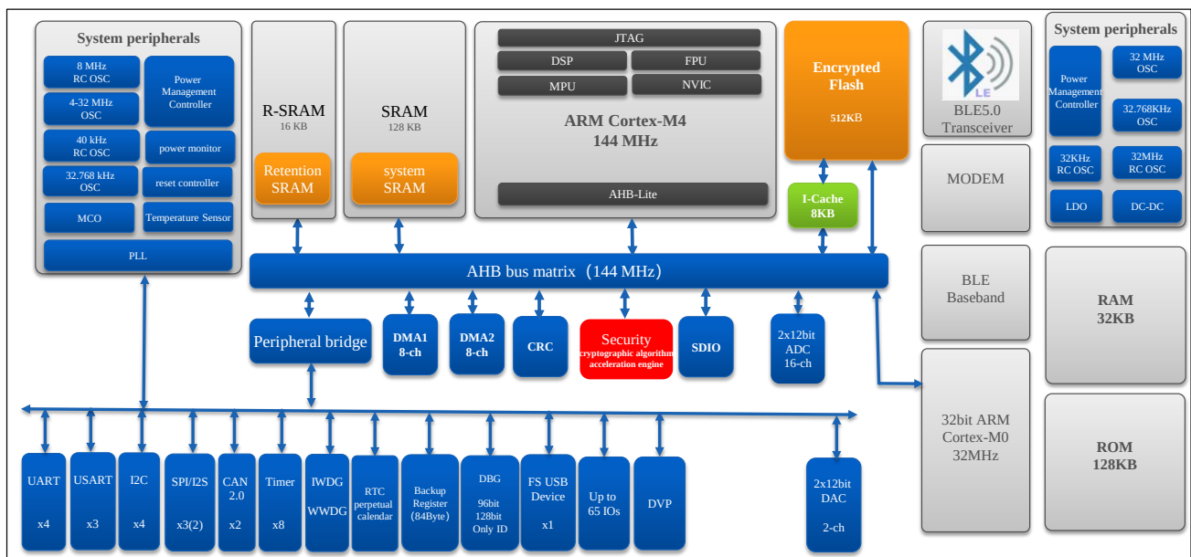
Figure 2-1 System principle diagram
