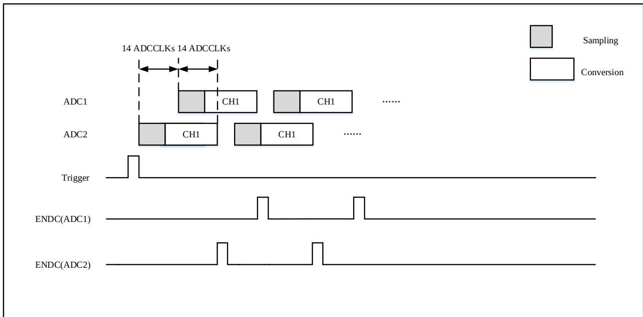
Figure 10-11 Schematic diagram of slow alternate mode conversion for 1 channel
