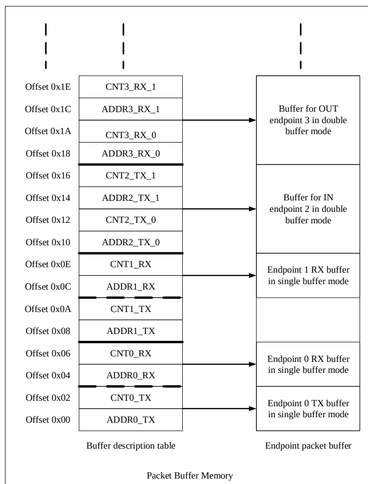
Figure 20-3 The relationship between the buffer description table and the endpoint packet buffer
