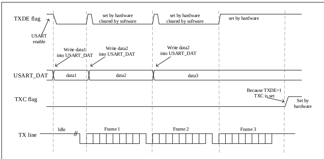
Figure 24-6 TXC/TXDE changes during transmission
