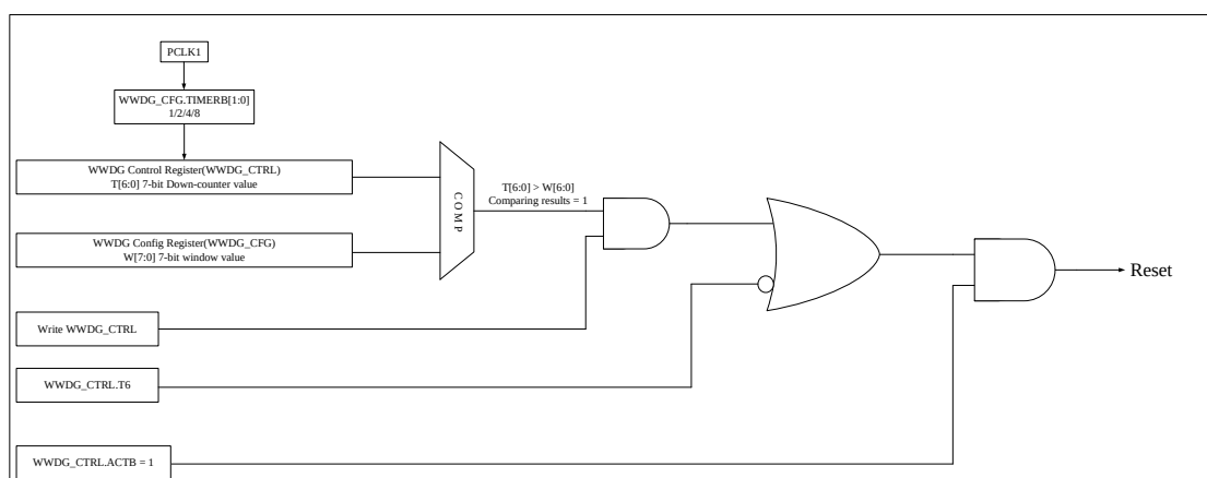
Figure 18-1 Watchdog block diagram
