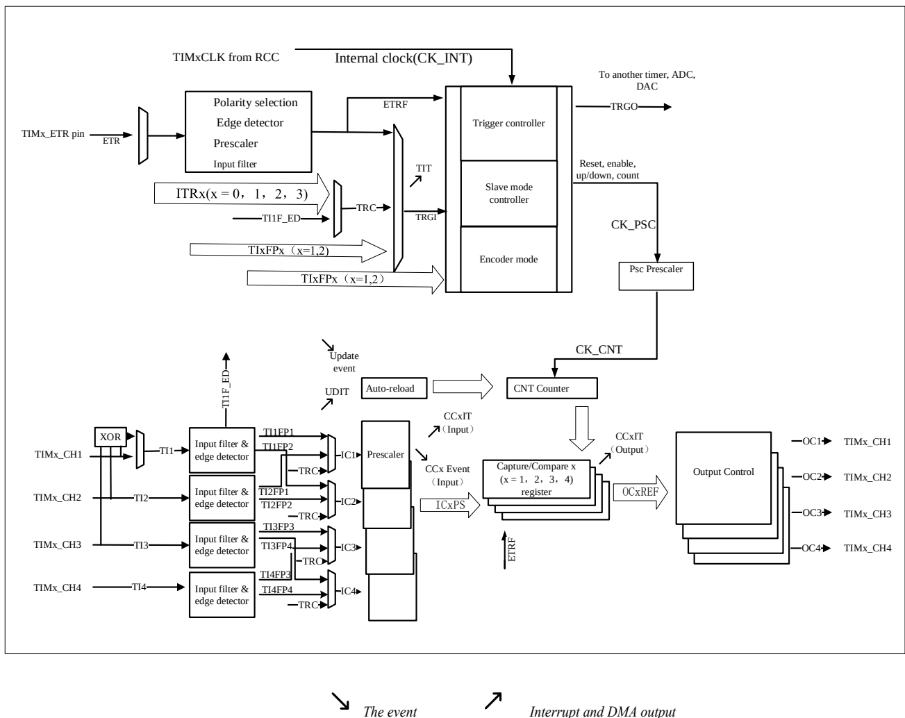
Figure 13-1 Block diagram of TIMx (x=2, 3, 4 and 5)
