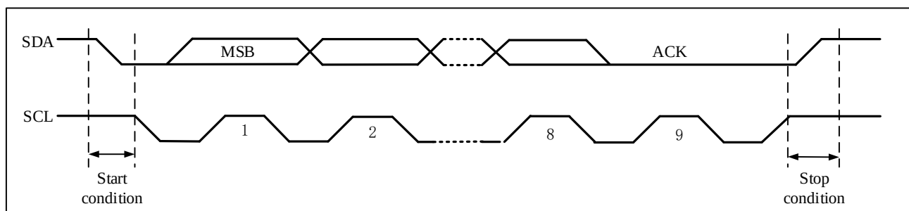
Figure 23-2 I2C bus protocol
