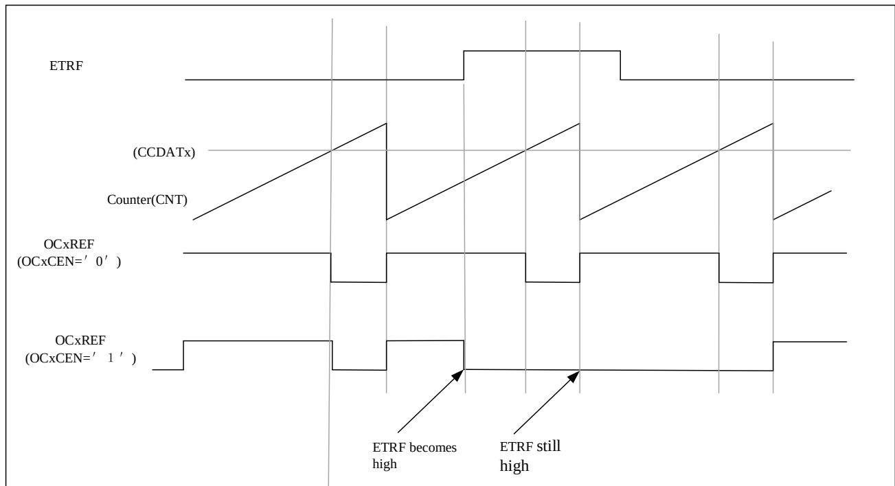
Figure 13-21 Control circuit in reset mode
