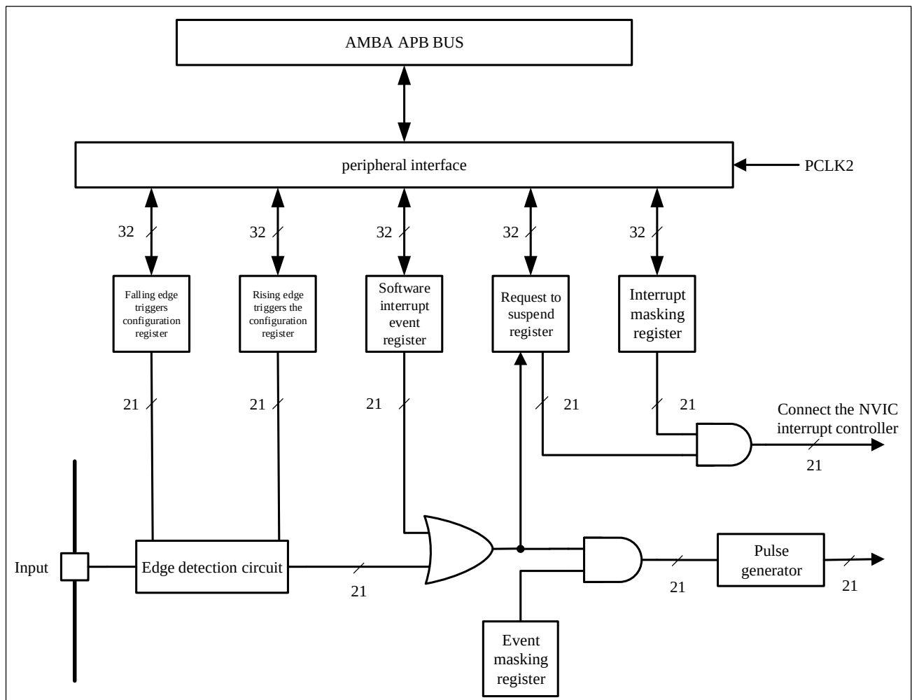
Figure 8-1 External interrupt/event controller block diagram
