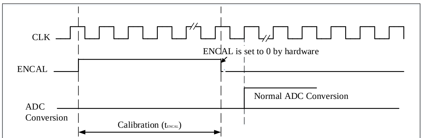
Figure 10-6 Calibration sequence diagram
