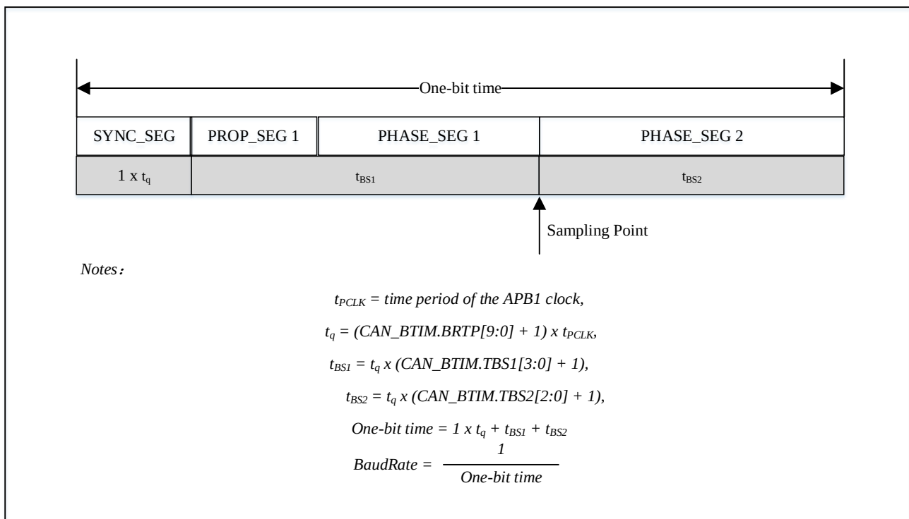
Figure 21-11 Bit sequence
