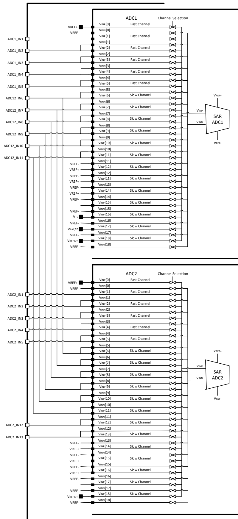
Figure 10-3 ADC1 and ADC2 channel pin connections
