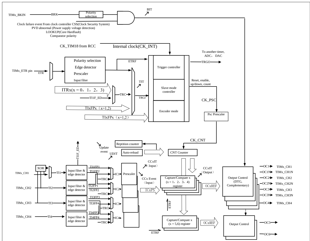
Figure 12-1 Block diagram of TIM1 and TIM8
