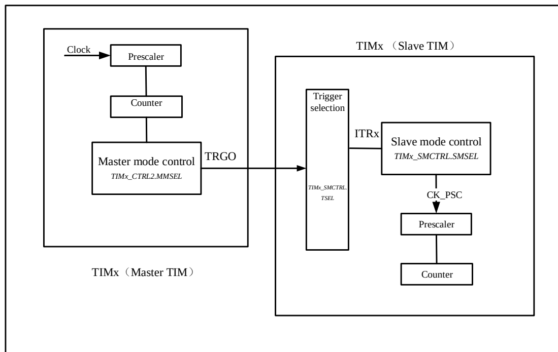
Figure 13-22 Block diagram of timer interconnection
