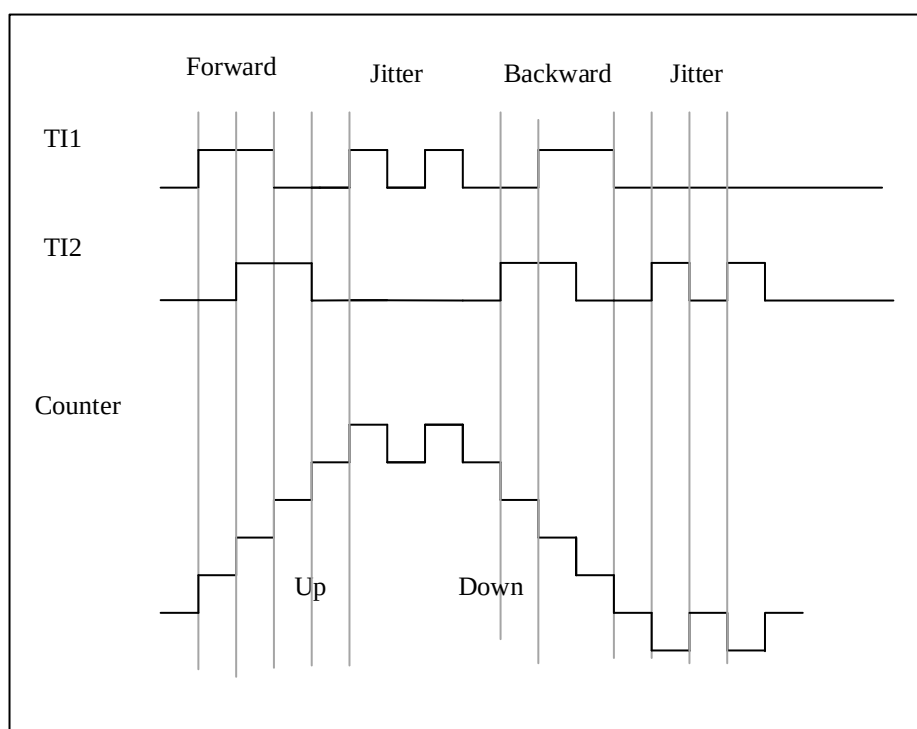
Figure 13-27 Example of counter operation in encoder interface mode
