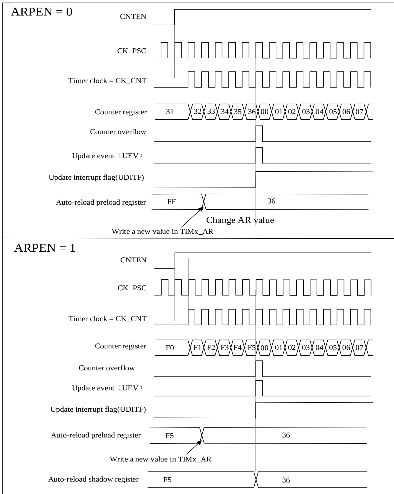
Figure 14-4 Timing diagram of the up-counting, update event when ARPEN=0/1
