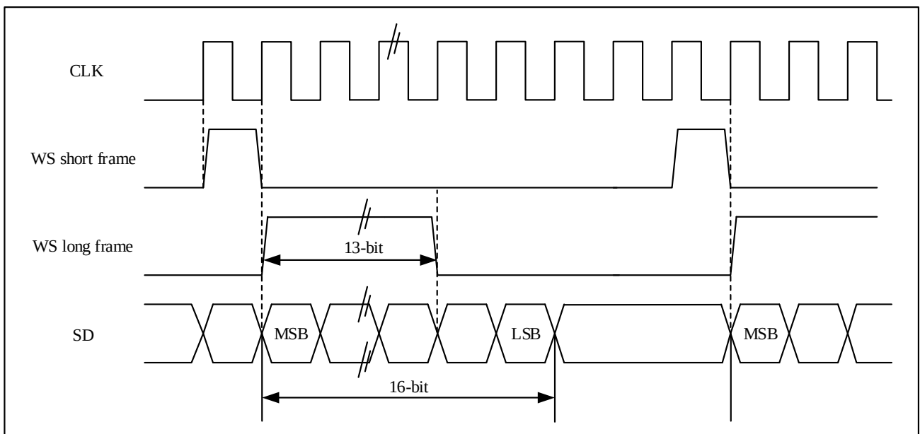
Figure 22-24 PCM standard waveform (16-bit extended to 32-bit packet frame)
