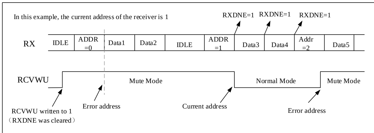
Figure 24-14 Mute mode detected using address mark
