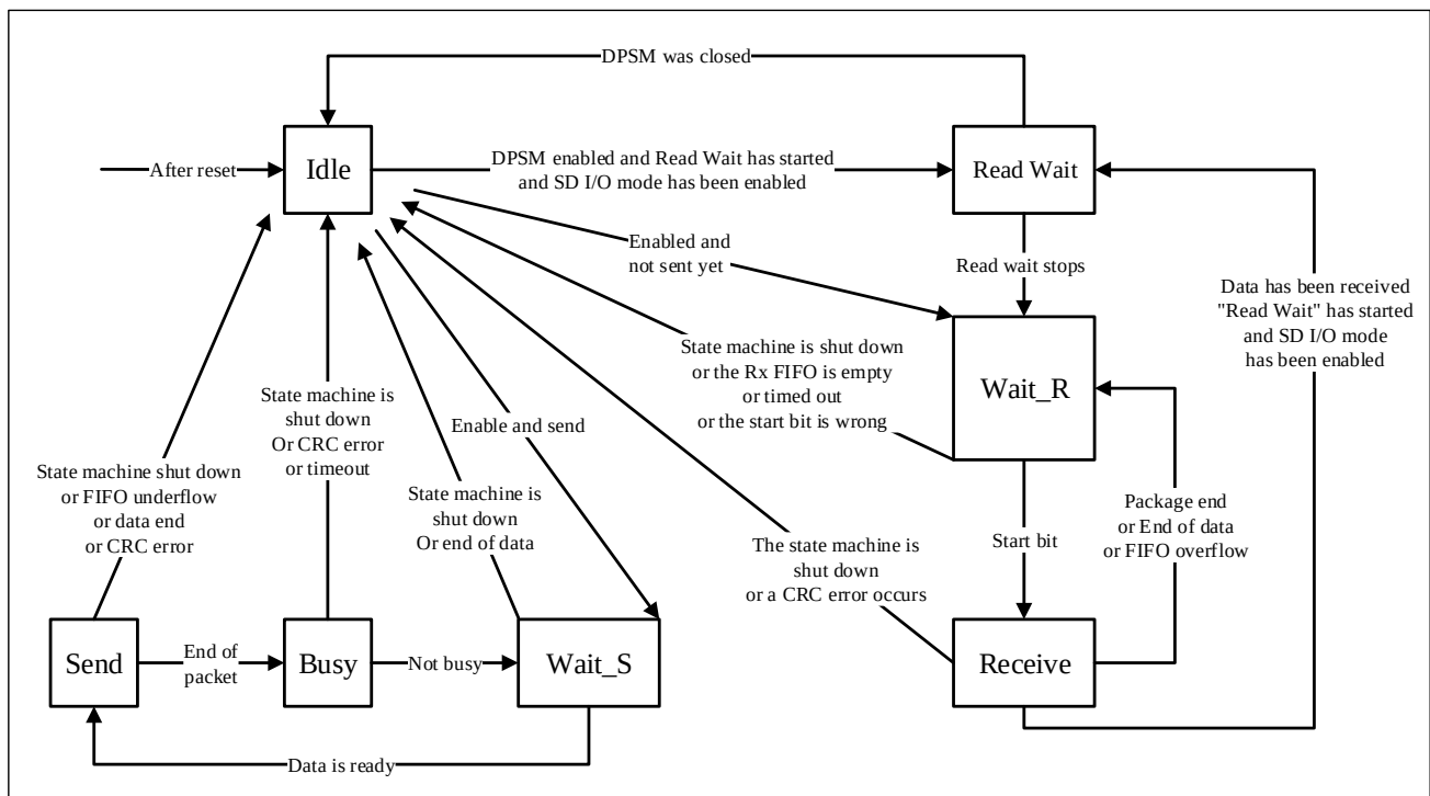
Figure 19-13 Data Path State Machine (DPSM)
