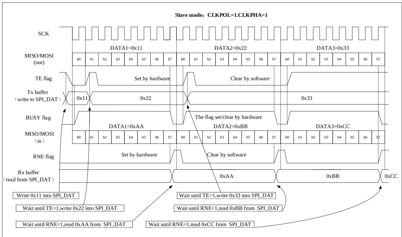
Figure 22-8 Schematic diagram of the change of TE/RNE/BUSY when the slave is continuously transmitting in full duplex mode
