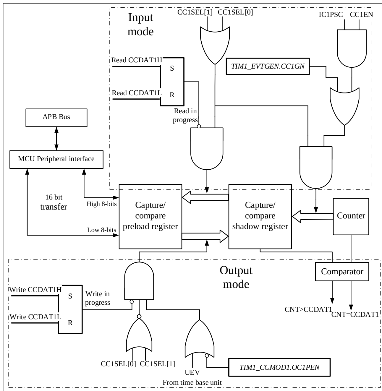
Figure 12-17 Capture/compare channel 1 main circuit
