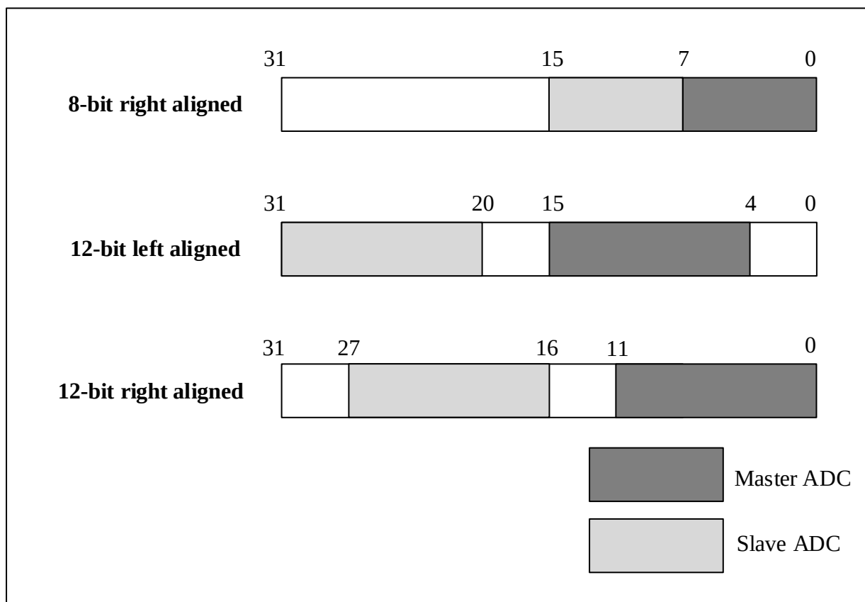
Figure 11-3 Data format for DAC sync output
