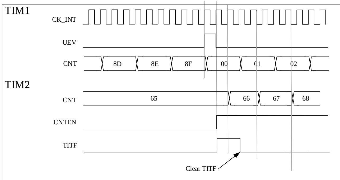
Figure 13-25 Trigger TIM2 with an update of TIM1
