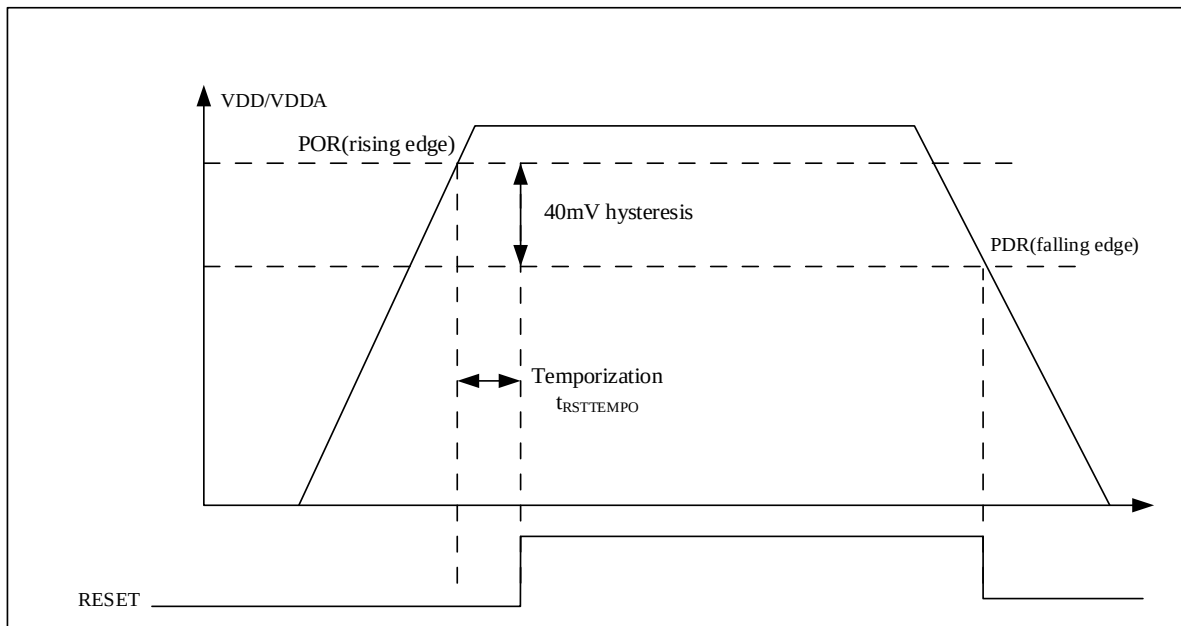
Figure 3-2 Waveforms of power-on reset and power-down reset
