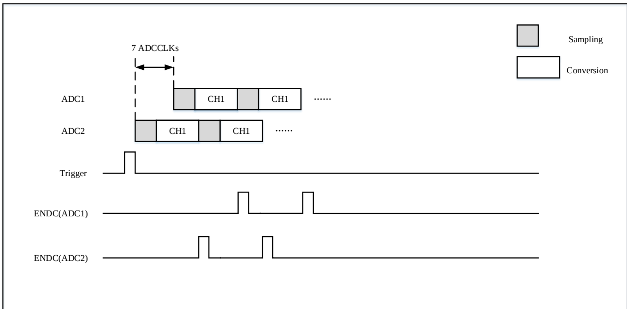
Figure 10-10 Schematic diagram of fast alternate mode conversion for continuous conversion of 1 channel
