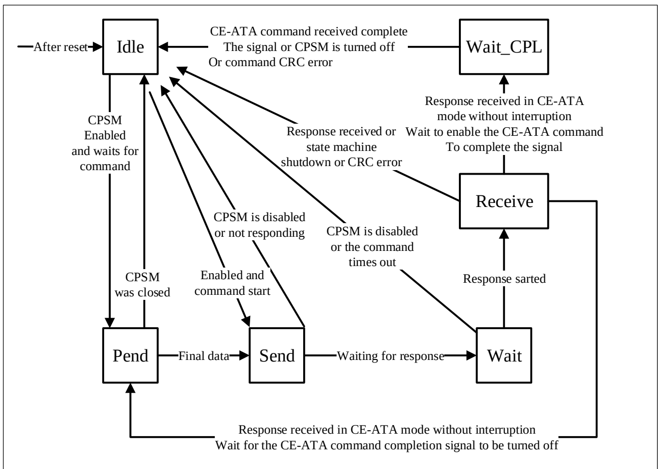
Figure 19-10 Command Path State Machine (CPSM)
