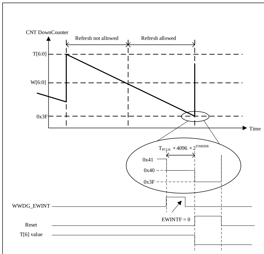
Figure 18-2 Refresh window and interrupt timing of WWDG
