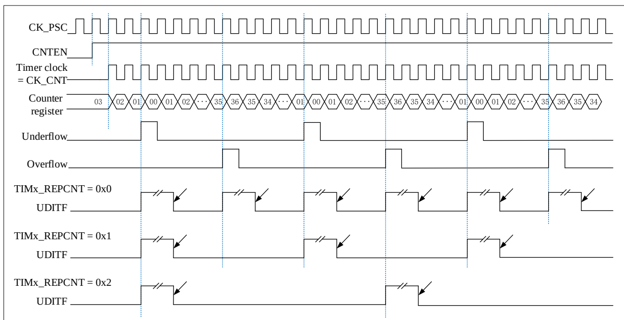
Figure 12-10 Repeat count sequence diagram in center-aligned mode
