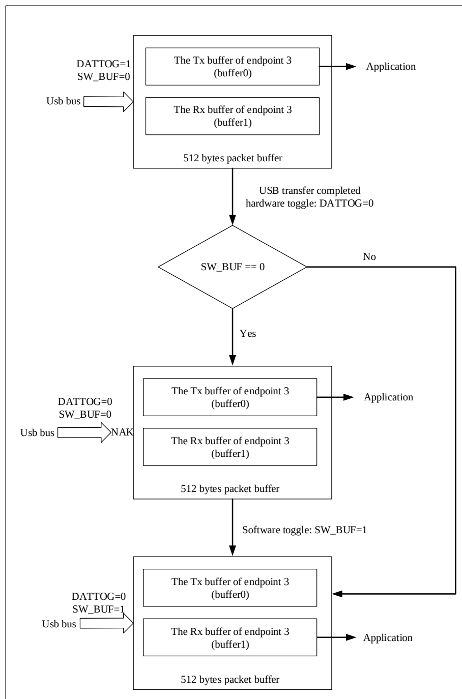
Figure 20-4 Double buffered bulk endpoint example
