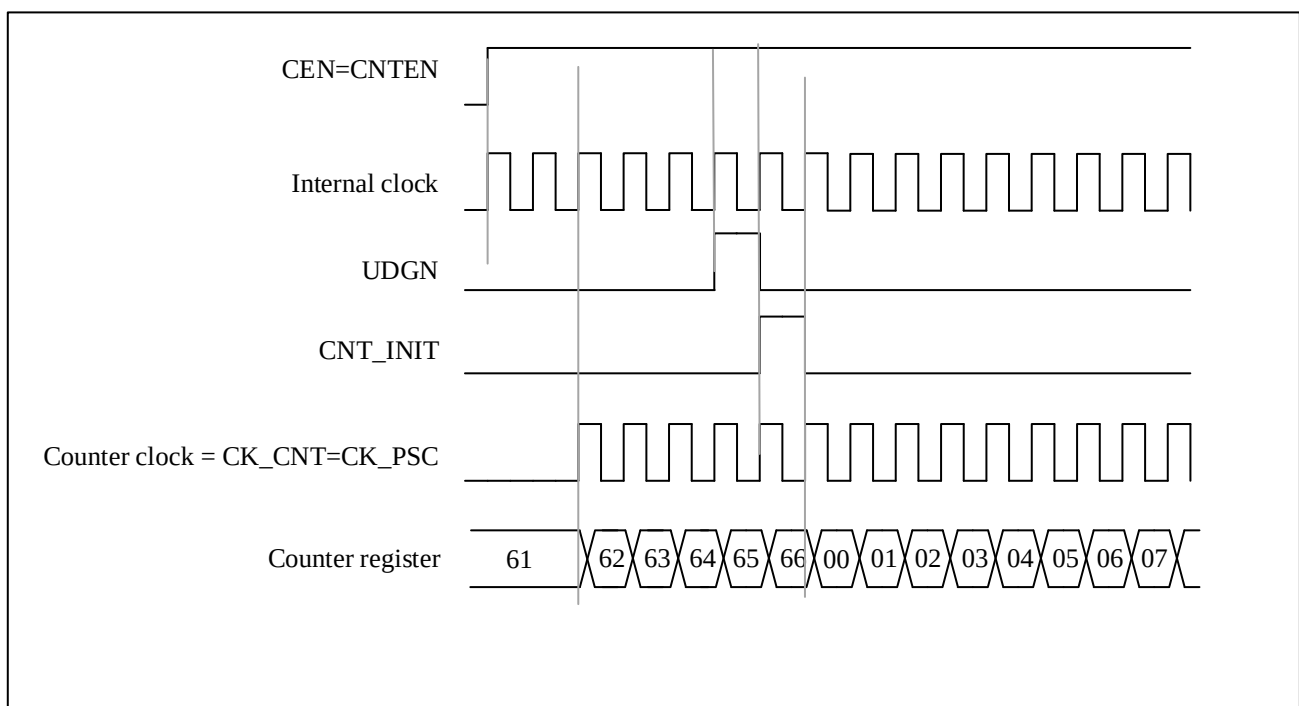
Figure 12-11 Control circuit in normal mode, internal clock divided by 1
