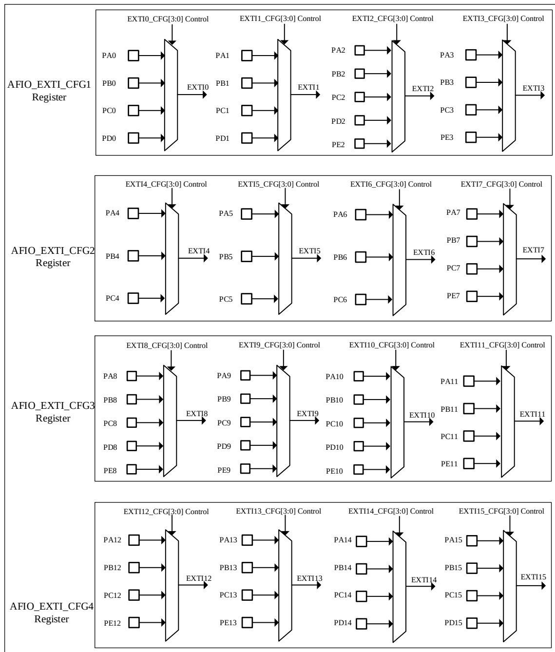
Figure 8-2 External interrupt GPIO mapping
