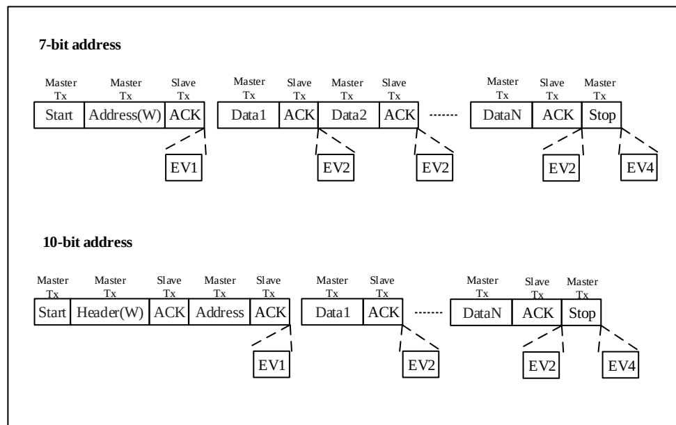
Figure 23-4 Slave receiver transfer sequence diagram
