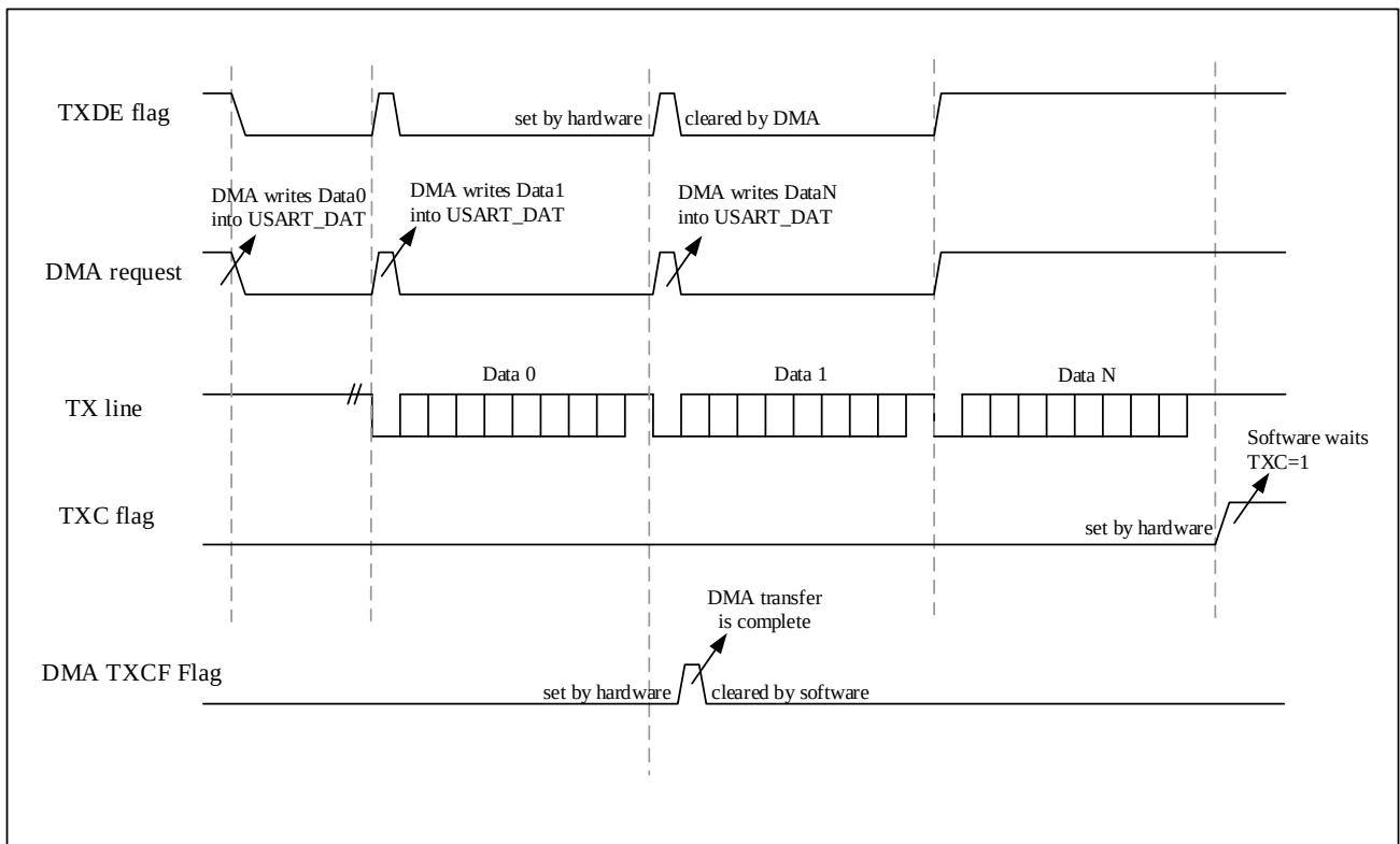
Figure 24-8 Transmission using DMA
