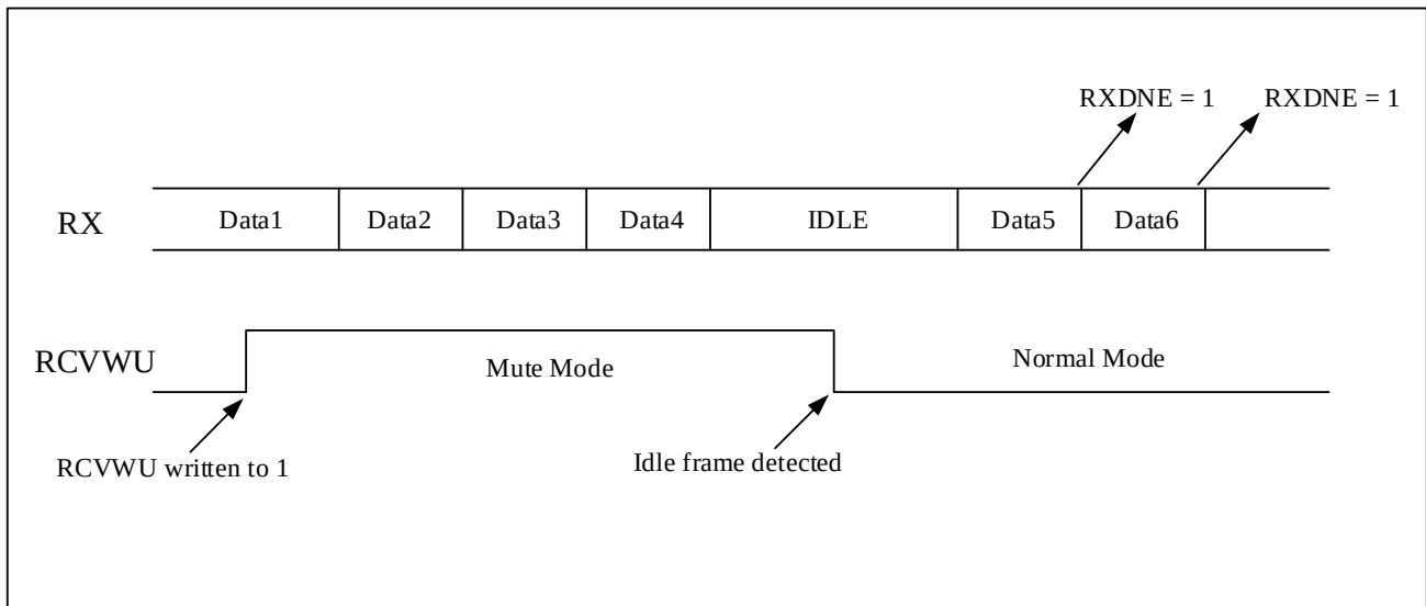
Figure 24-13 Mute mode using idle line detection
