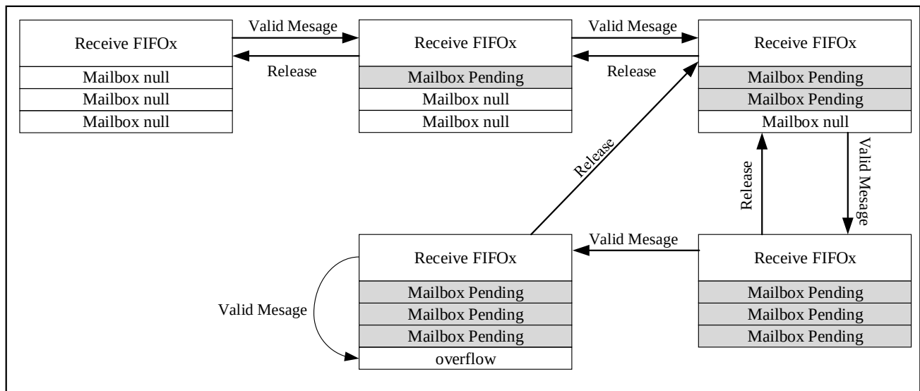
Figure 21-8 Receive FIFO status
