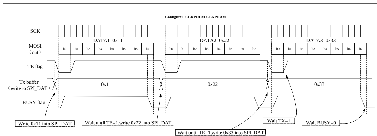
Figure 22-10 Schematic diagram of TE/BUSY change when BIDIRMODE = 0 and RONLY = 0 are transmitted discontinuously.
