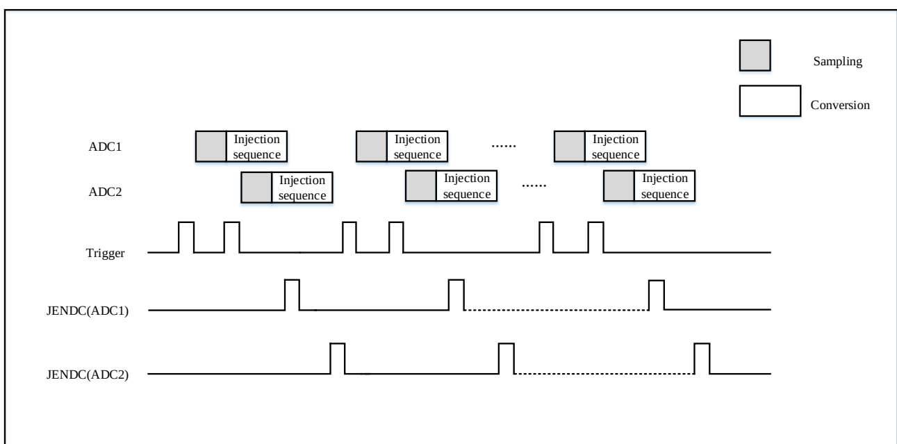
Figure 10-12 Rotation triggering: injecting channel groups
