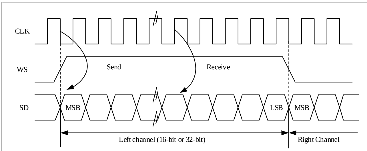
Figure 22-18 MSB aligns 24-bit data, CLKPOL = 0
