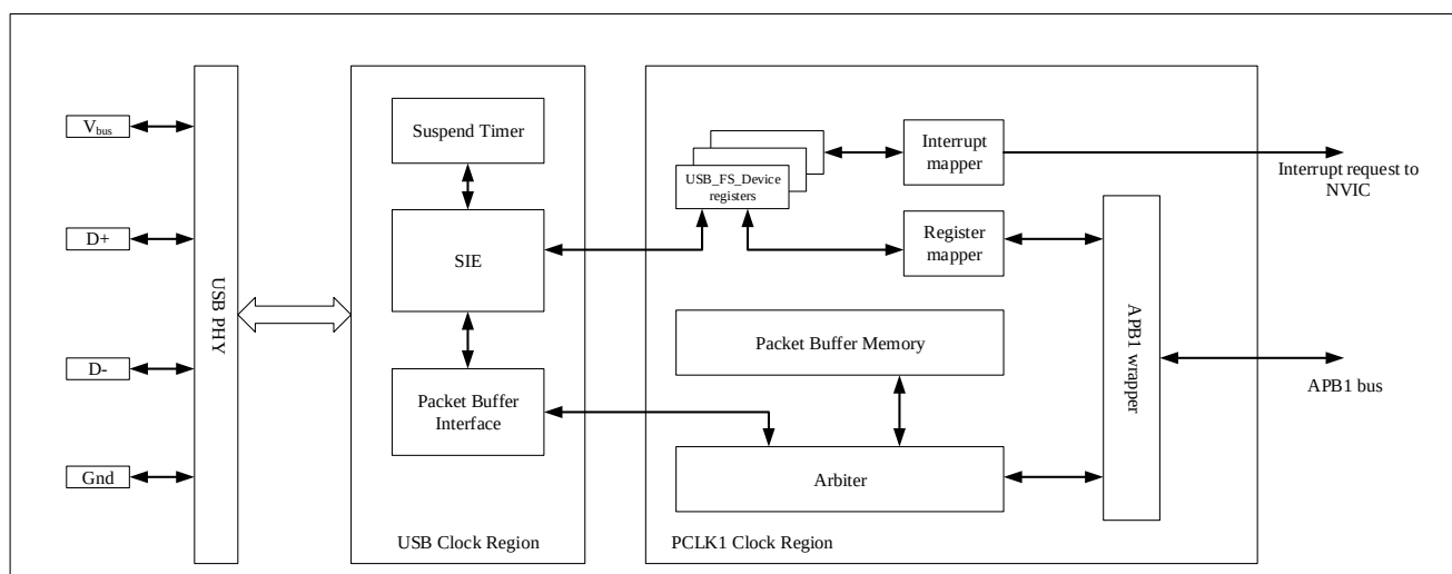
Figure 20-1 USB device block diagram
