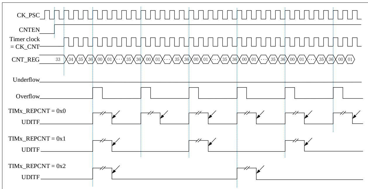
Figure 12-9 Repeat count sequence diagram in up-counting mode
