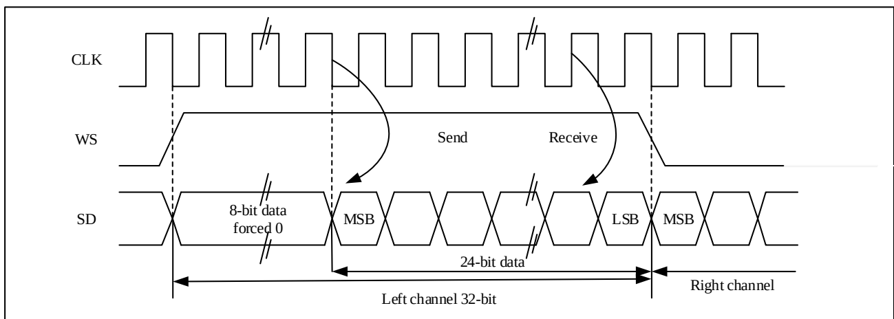
Figure 22-21 LSB aligns 24-bit data, CLKPOL = 0
