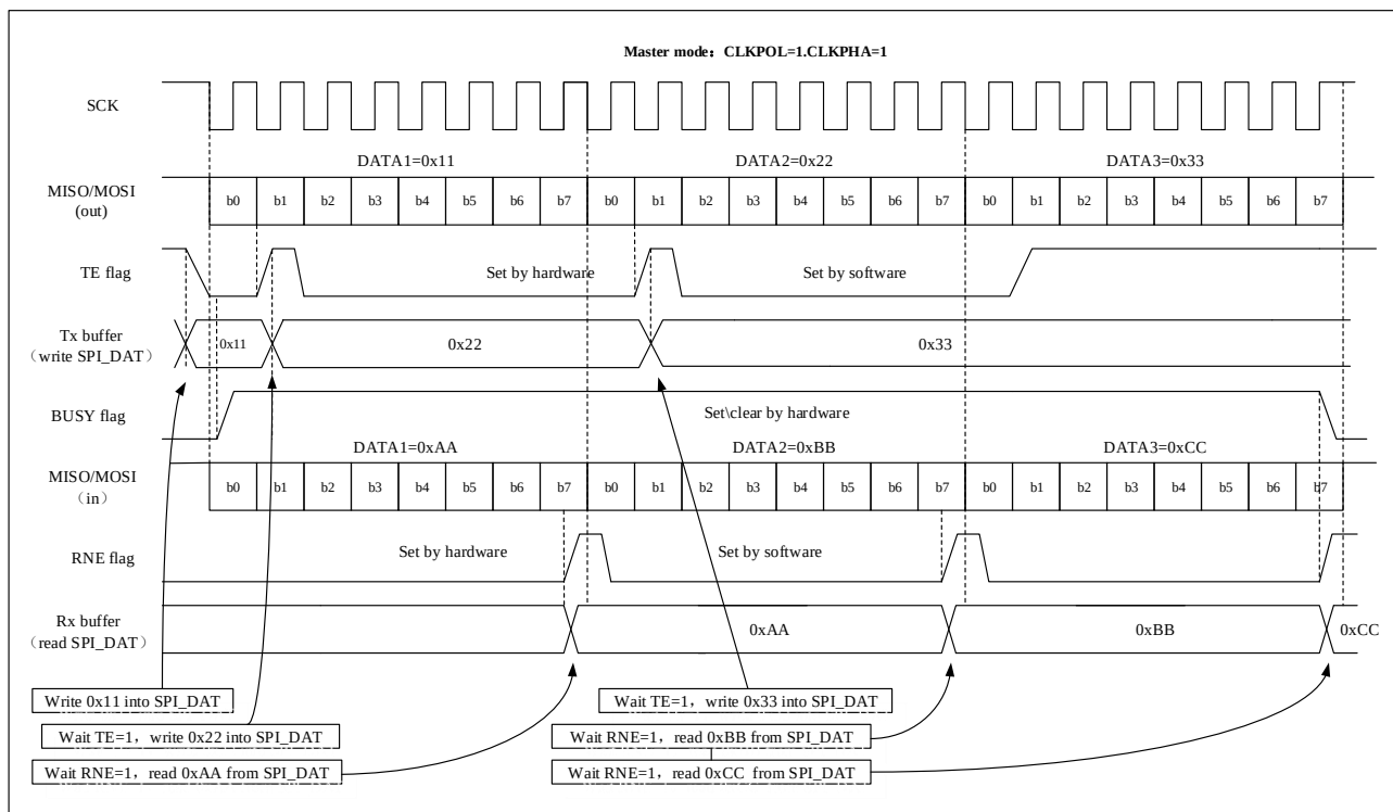
Figure 22-5 Schematic diagram of the change of TE/RNE/BUSY when the host is continuously transmitting in full duplex mode
