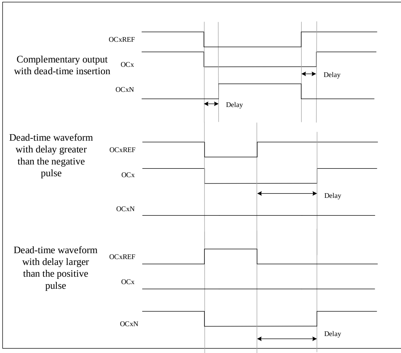
Figure 12-25 Complementary output with dead-time insertion
