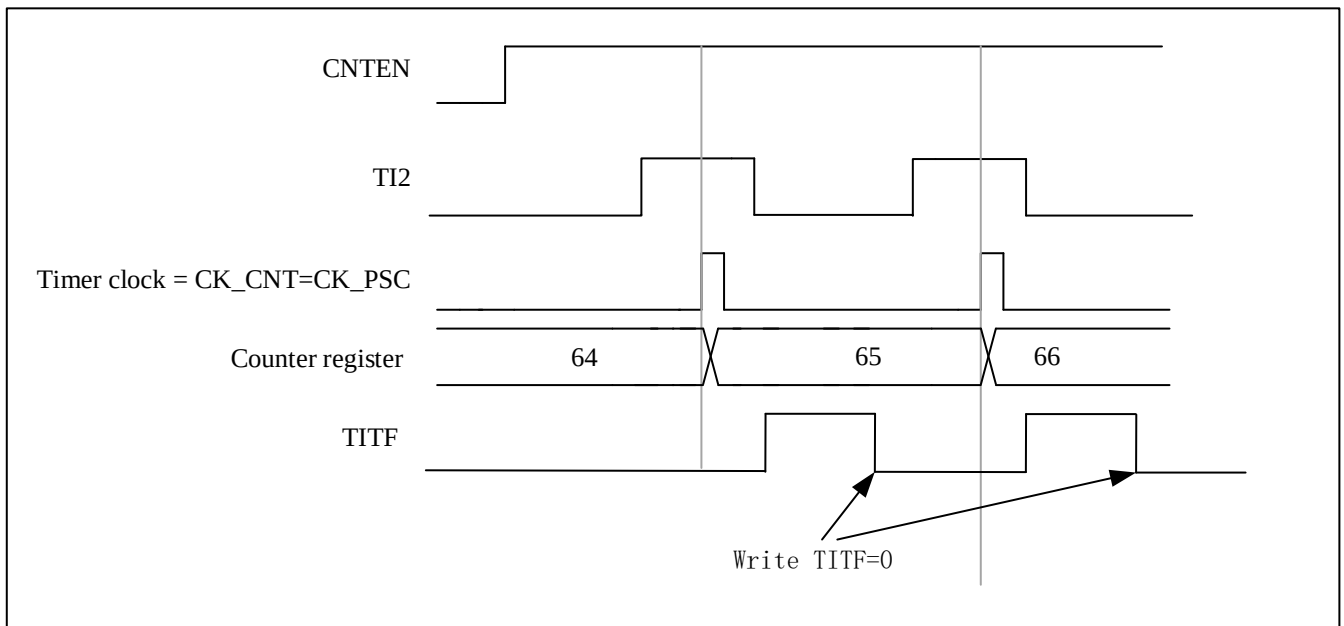
Figure 12-13 Control circuit in external clock mode 1
