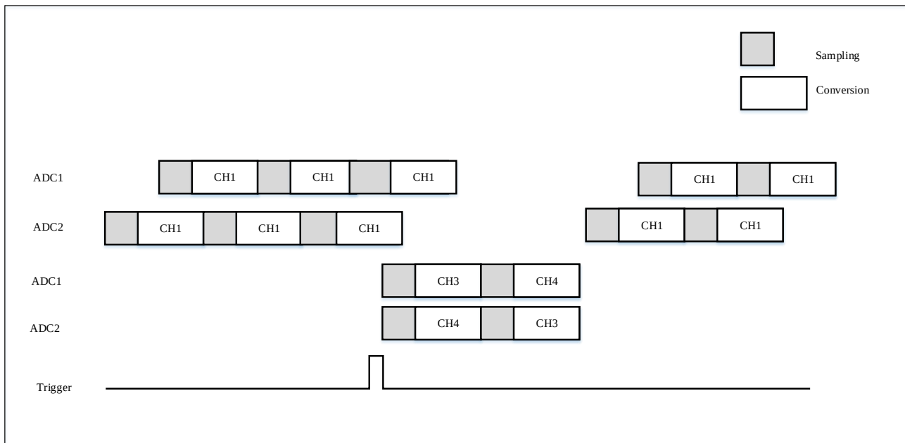
Figure 10-16 Alternate single-channel conversions are interrupted by injection sequences CH3 and CH4
