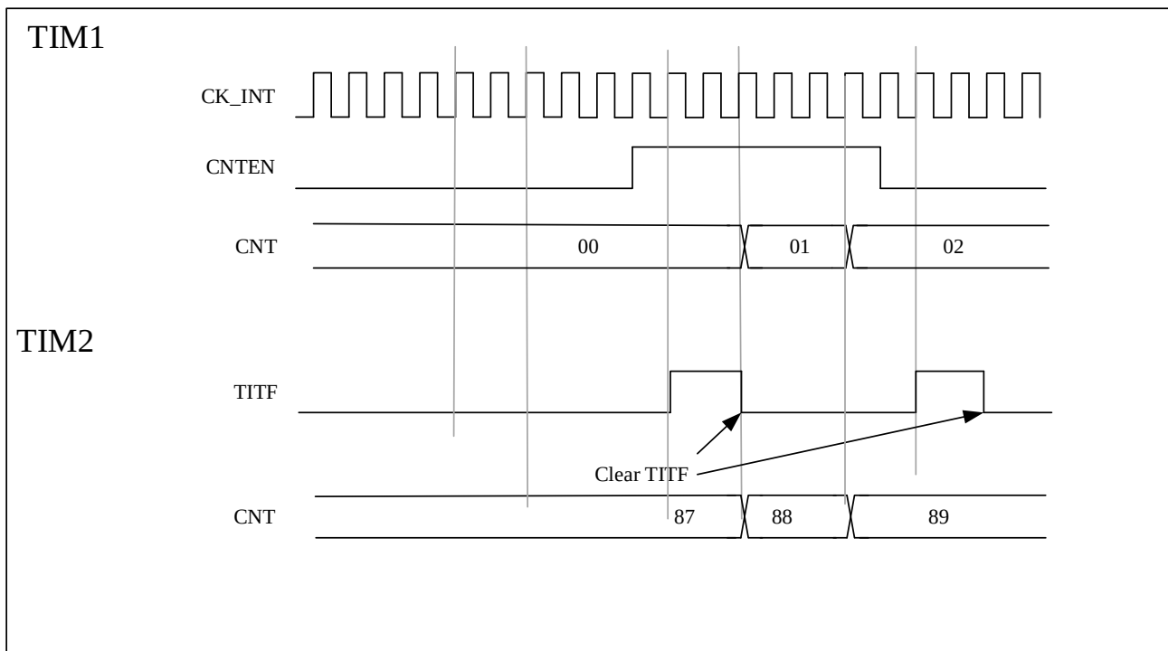
Figure 13-24 TIM2 gated by enable signal of TIM1
