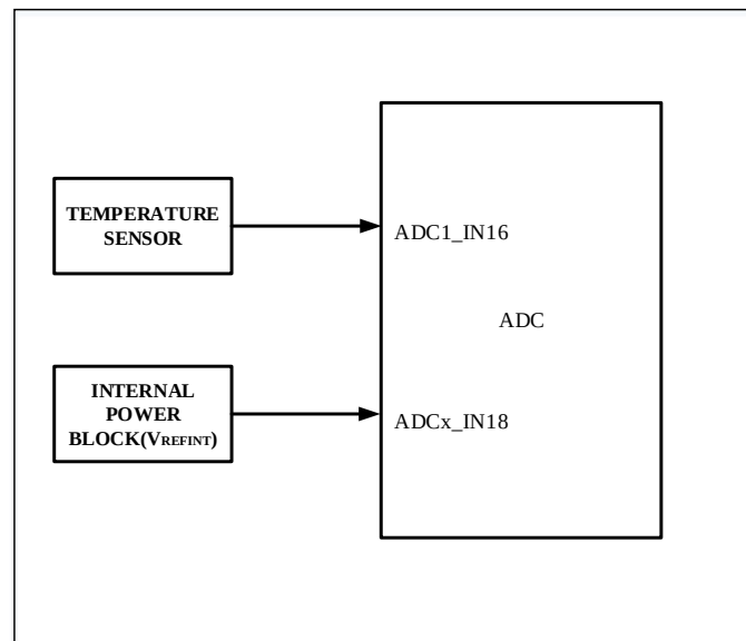
Figure 10-17 Temperature sensor and VREFINT diagram of the channel
