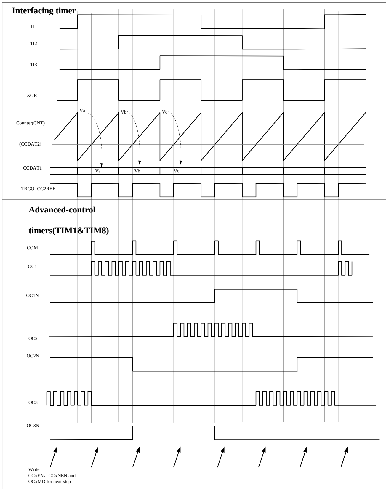
Figure 12-34 Example of Hall sensor interface
