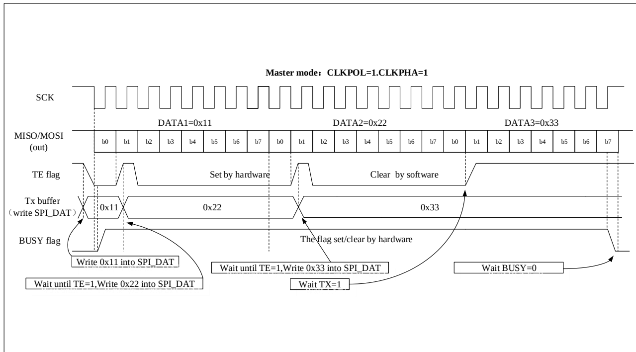
Figure 22-6 Schematic diagram of TE/BUSY change when the host transmits continuously in one-way only mode
