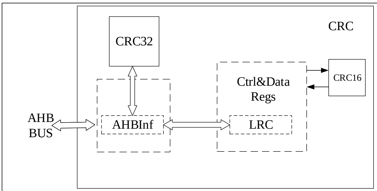
Figure 16-1 CRC calculation unit block diagram
