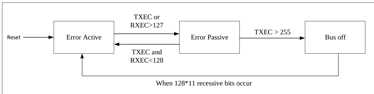
Figure 21-14 CAN error state diagram
