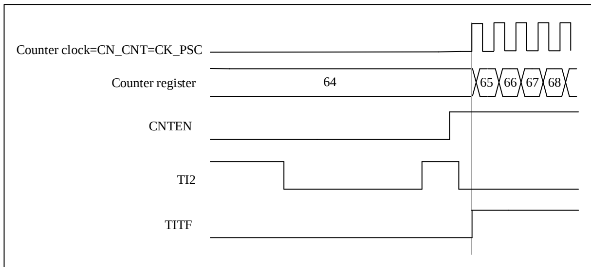
Figure 12-28 Control circuit in Trigger mode
