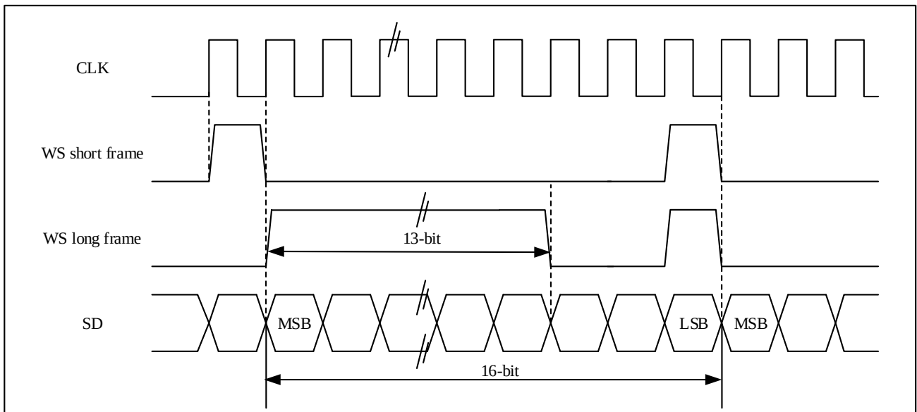
Figure 22-24 PCM standard waveform (16-bit extended to 32-bit packet frame)
