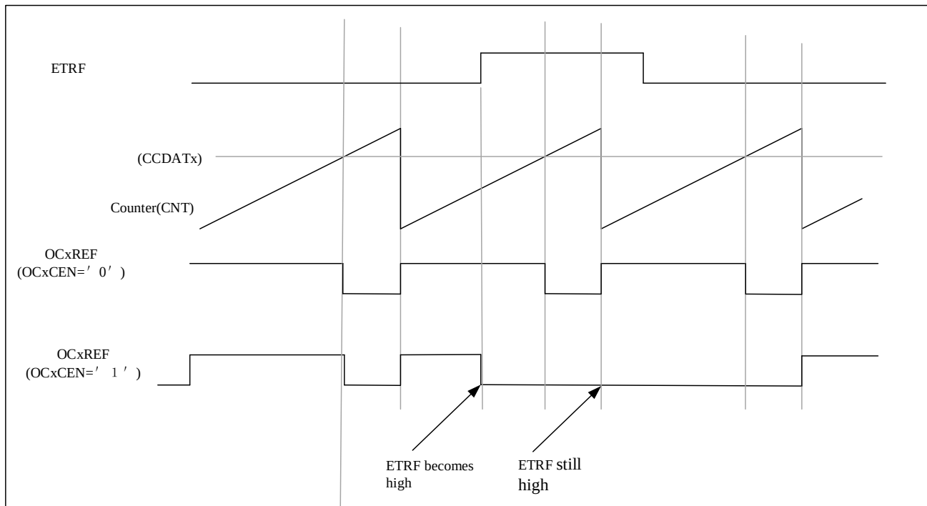
Figure 12-24 Clearing the OCxREF of TIMx
