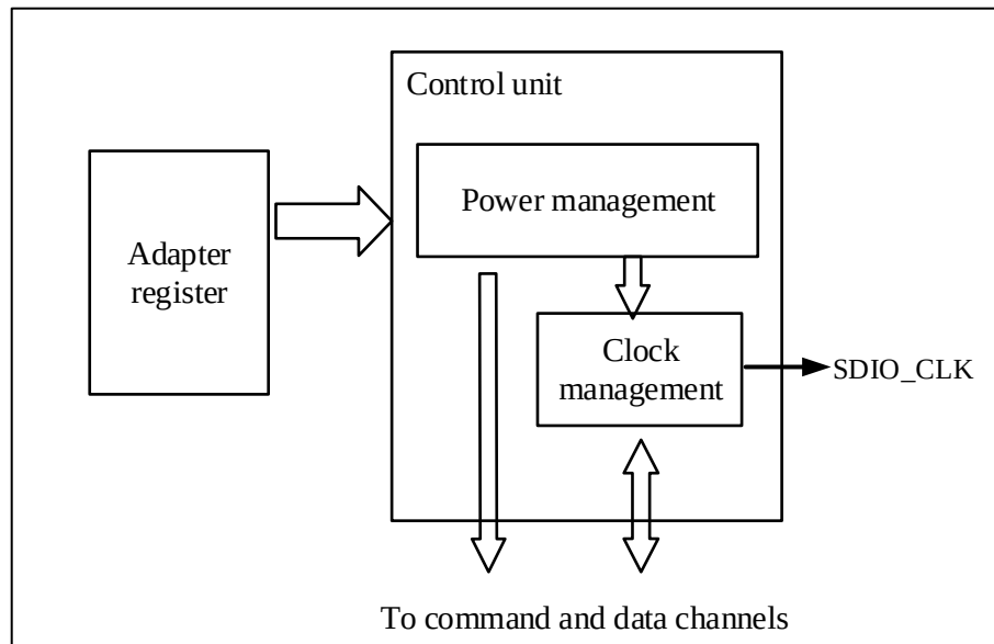
Figure 19-8 Control unit
