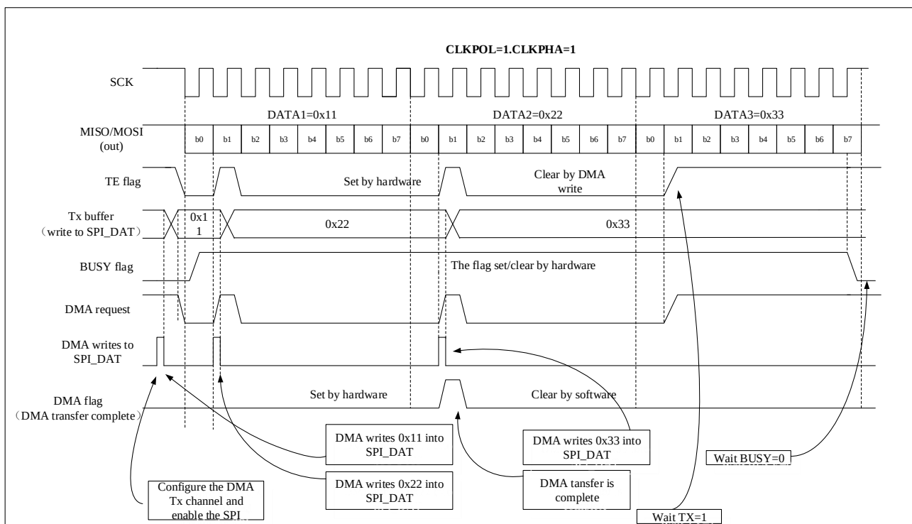
Figure 22-11 Transmission using DMA
