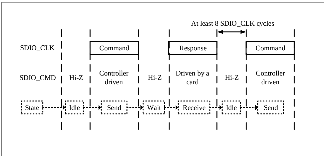
Figure 19-11 SDIO command transmission
