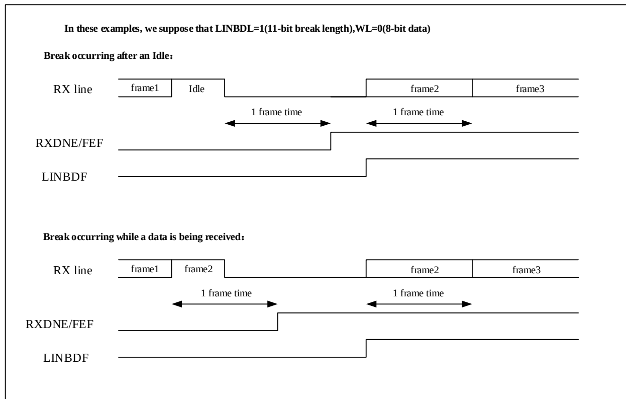
Figure 24-22 Break detection and framing error detection in LIN mode
