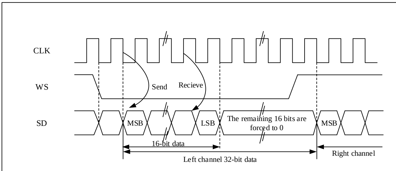
Figure 22-16 I 2 S Philips protocol standard waveform (16-bit extended to 32-bit packet frame, CLKPOL = 0)
