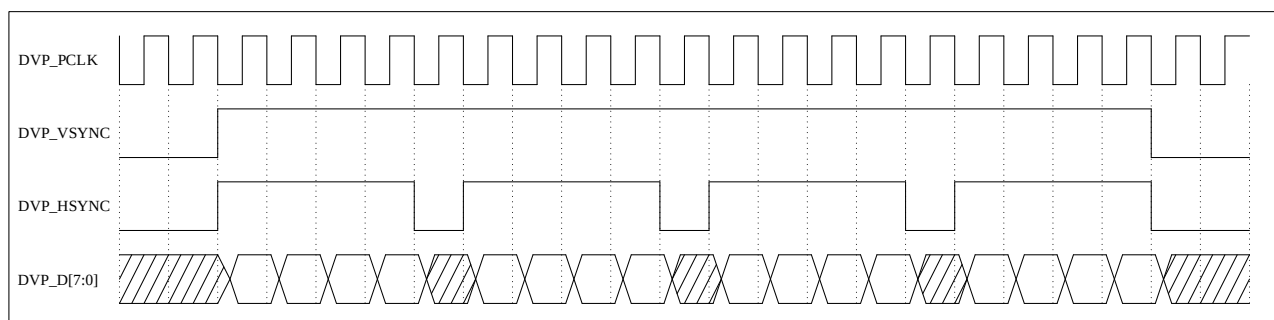
Figure 25-1 DVP interface timing example
