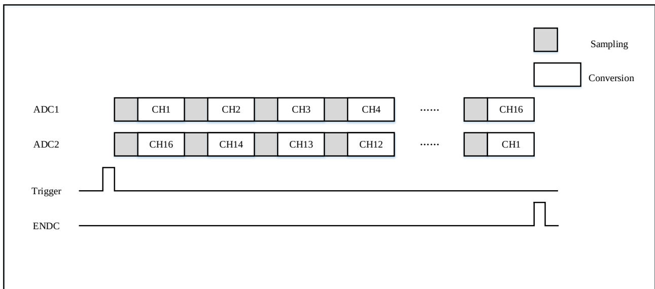
Figure 10-8 Schematic diagram of synchronous regular mode conversion of 16 channels
