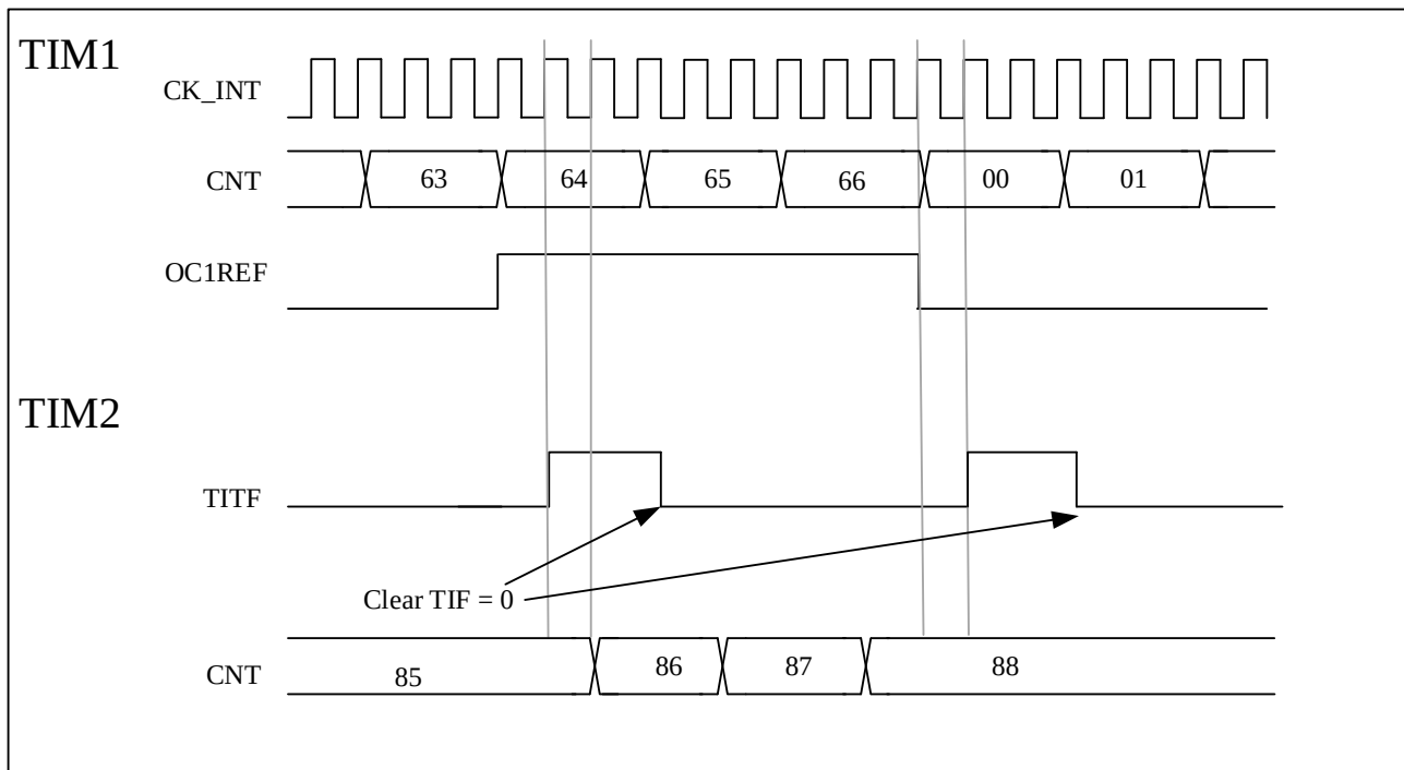
Figure 13-23 TIM2 gated by OC1REF of TIM1
