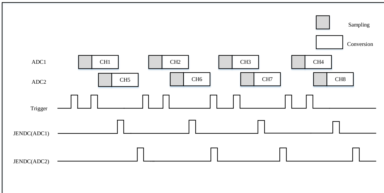
Figure 10-13 Rotation trigger: inject channel group in discontinuous mode
