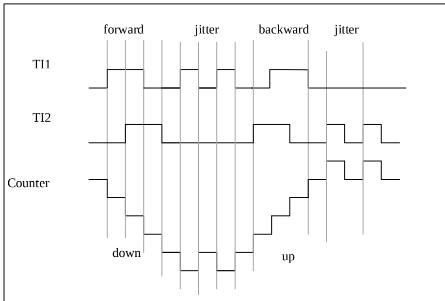
Figure 13-28 Encoder interface mode example with IC1FP1 polarity inverted
