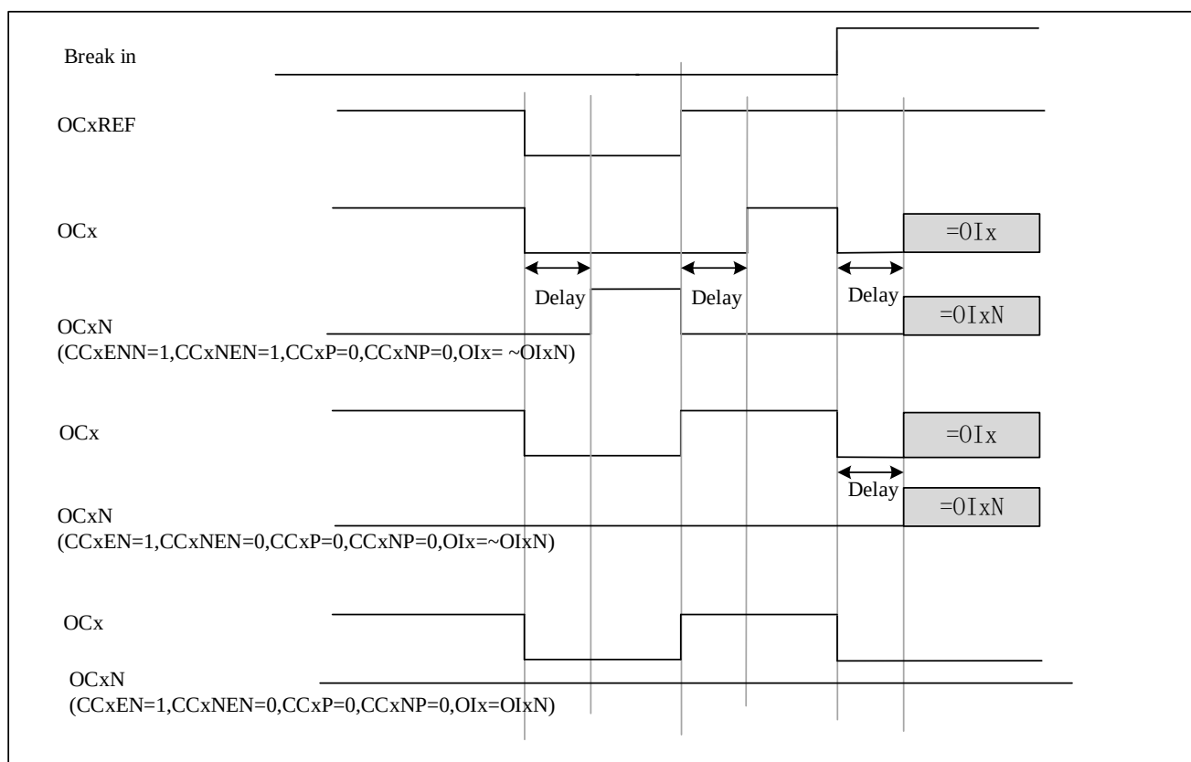
Figure 12-26 Output behavior in response to a break
