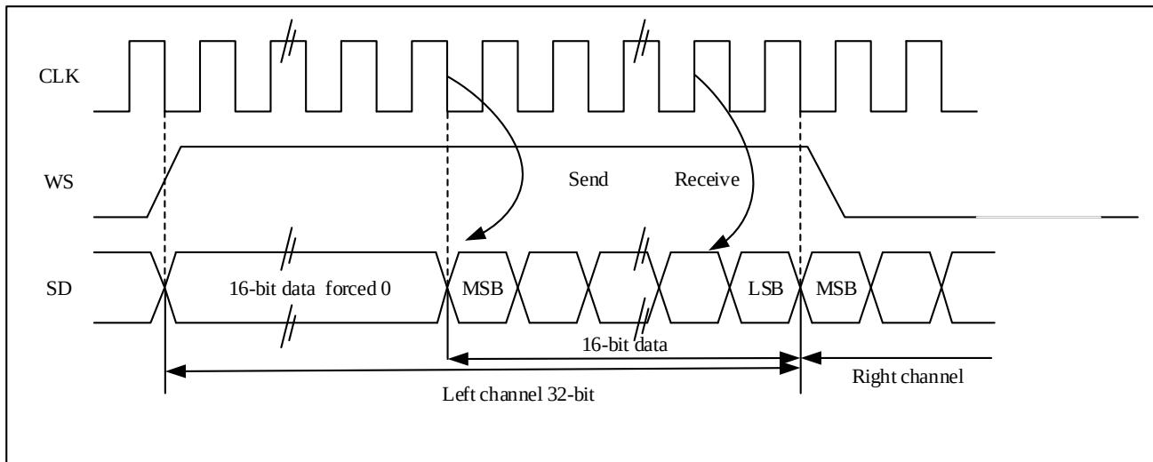
Figure 22-22 LSB aligned 16-bit data is extended to 32-bit packet frame, CLKPOL = 0
