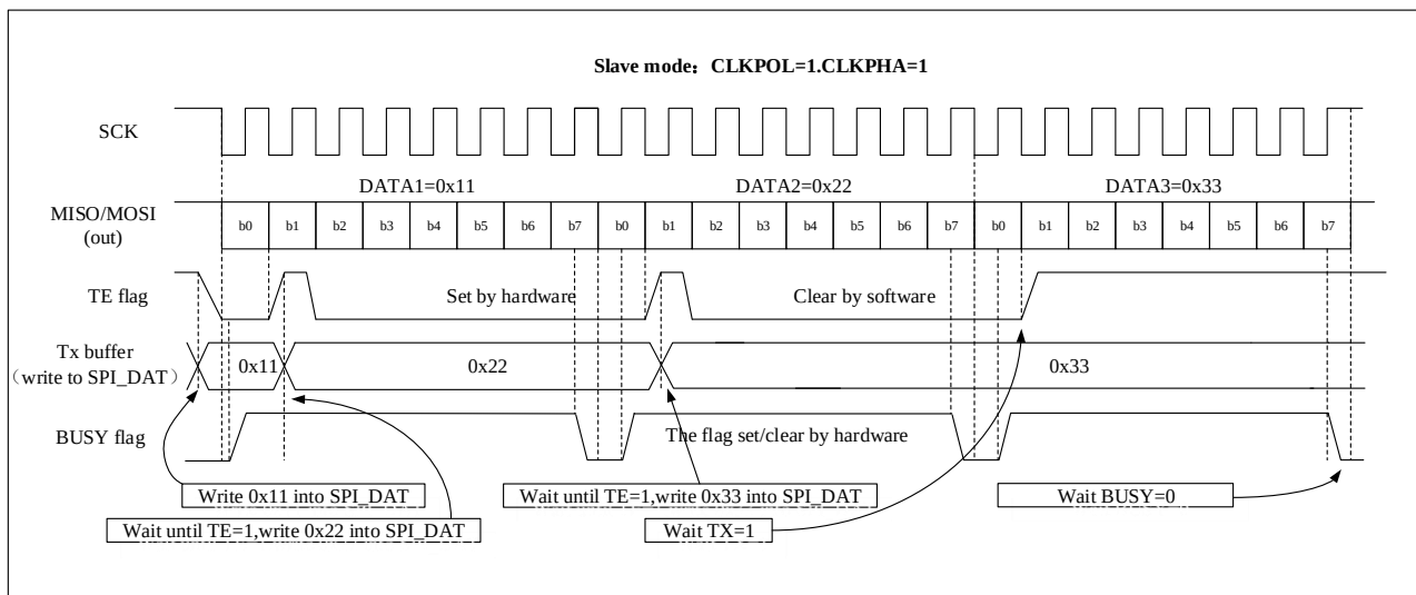
Figure 22-9 Schematic diagram of TE/BUSY change during continuous transmission in slave unidirectional transmit-only mode
