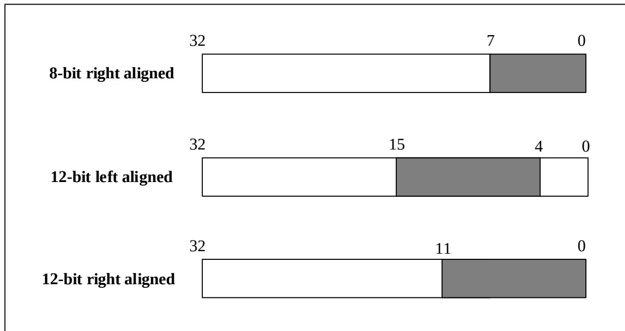
Figure 11-2 Data format when DAC independent output
