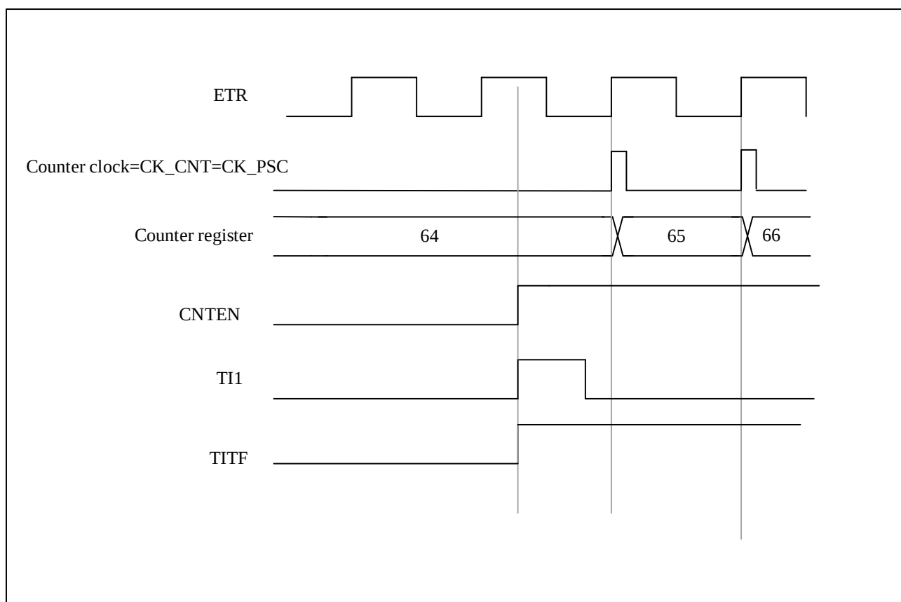
Figure 12-30 Control circuit in Trigger Mode + External Clock Mode2
