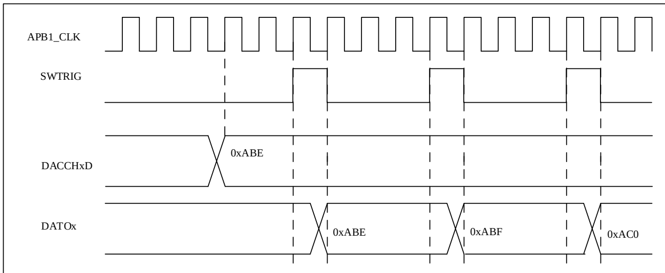
Figure 11-8 DAC conversion with trigonometry generation (enable software trigger)
