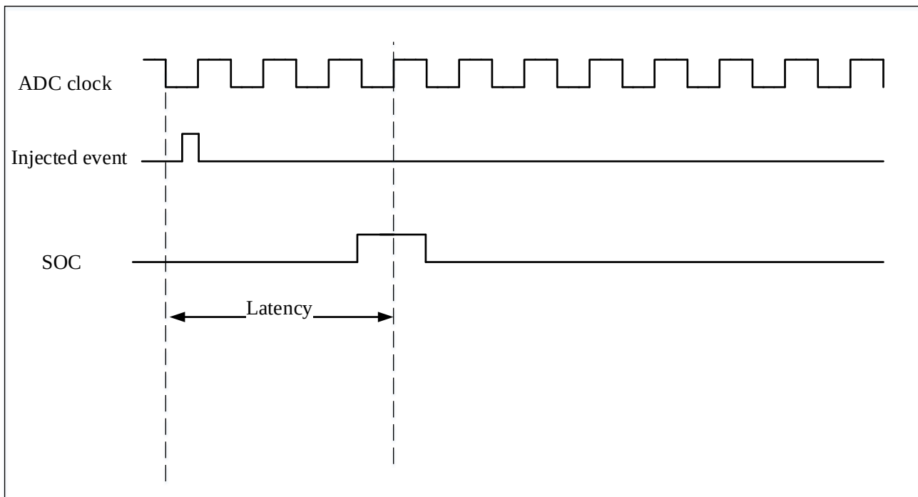
Figure 10-5 Injection conversion delay
