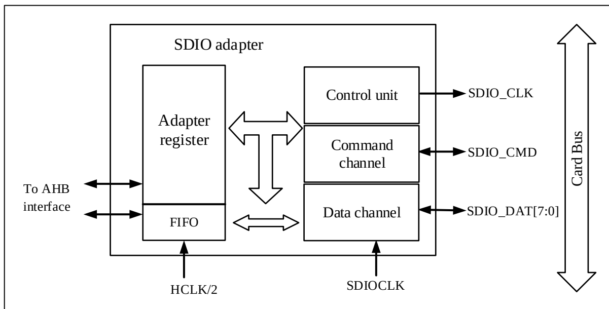
Figure 19-7 SDIO adapter
