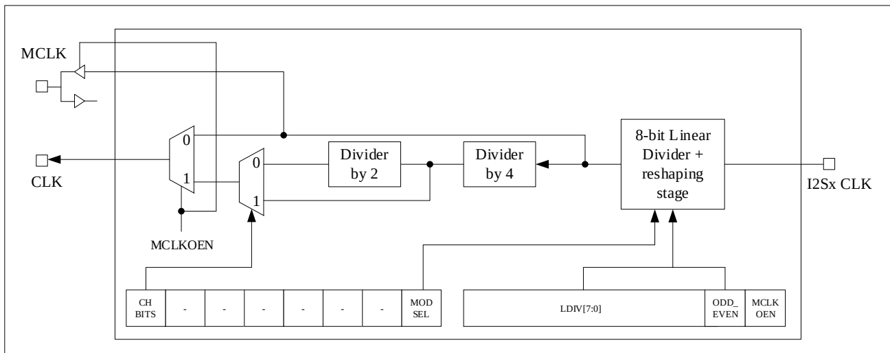
Figure 22-25 I 2 S clock generator structure
