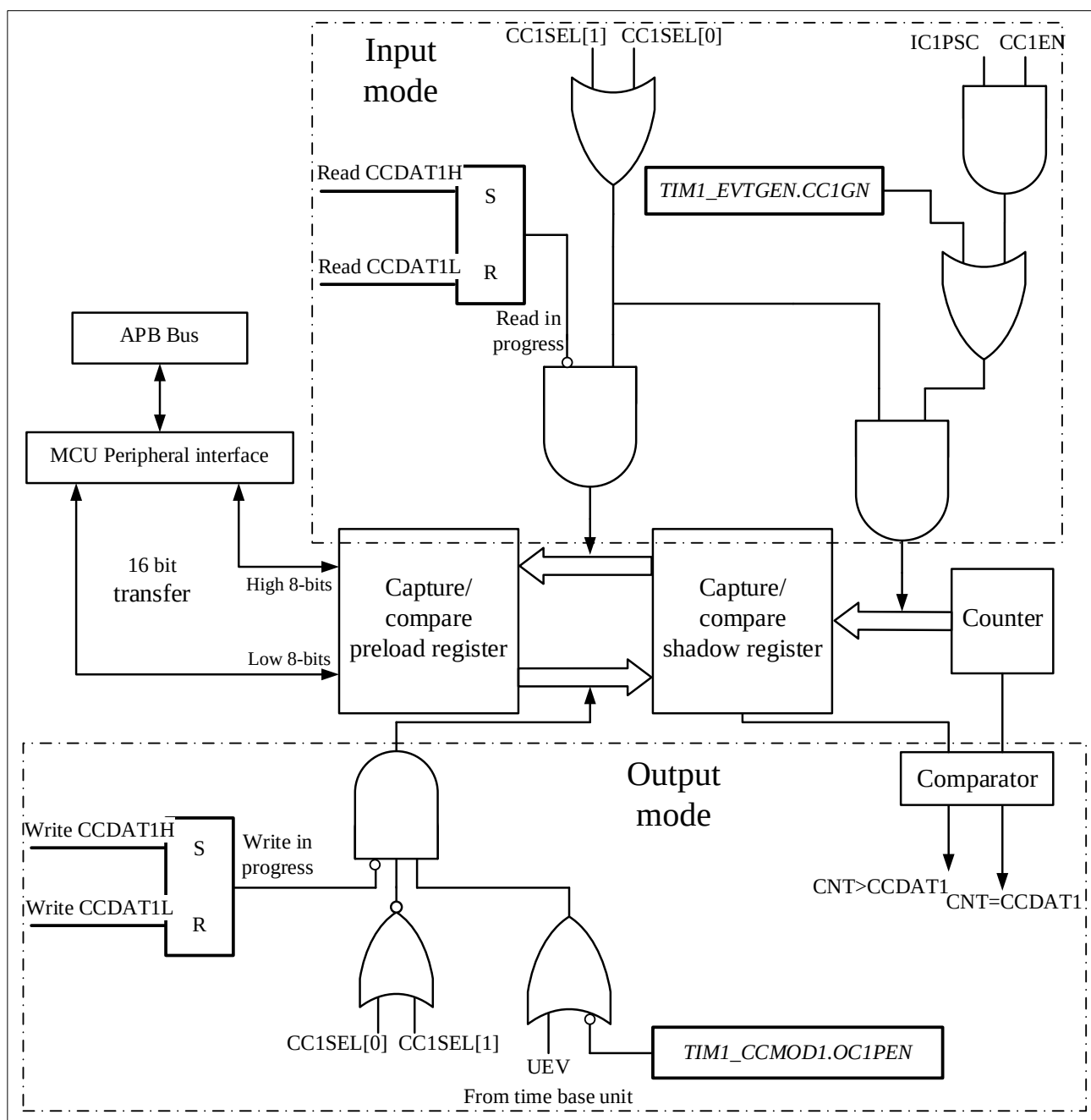
Figure 13-14 Capture/compare channel 1 main circuit
