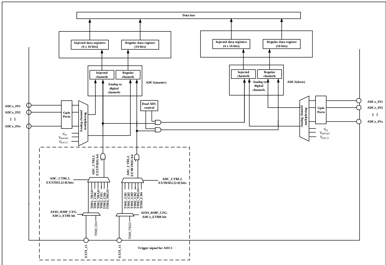
Figure 10-7 Dual ADC Block Diagram
