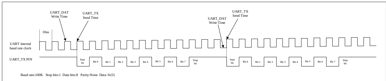
Figure 24-5 Transmission time difference
