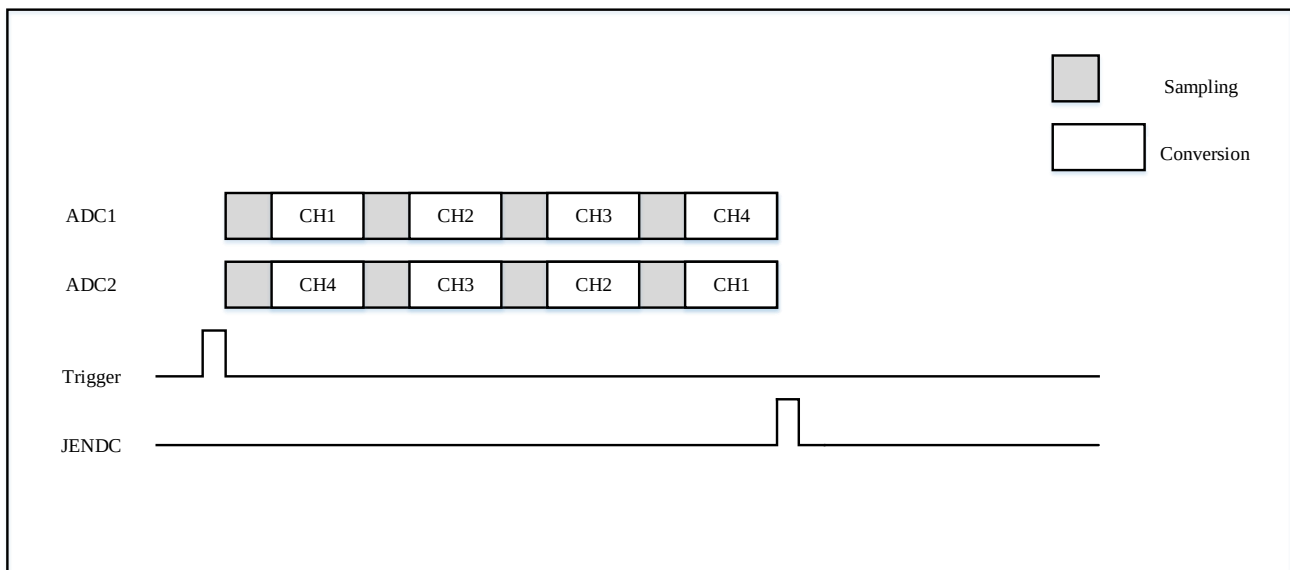
Figure 10-9 Schematic diagram of synchronous injection mode conversion of 4 channels
