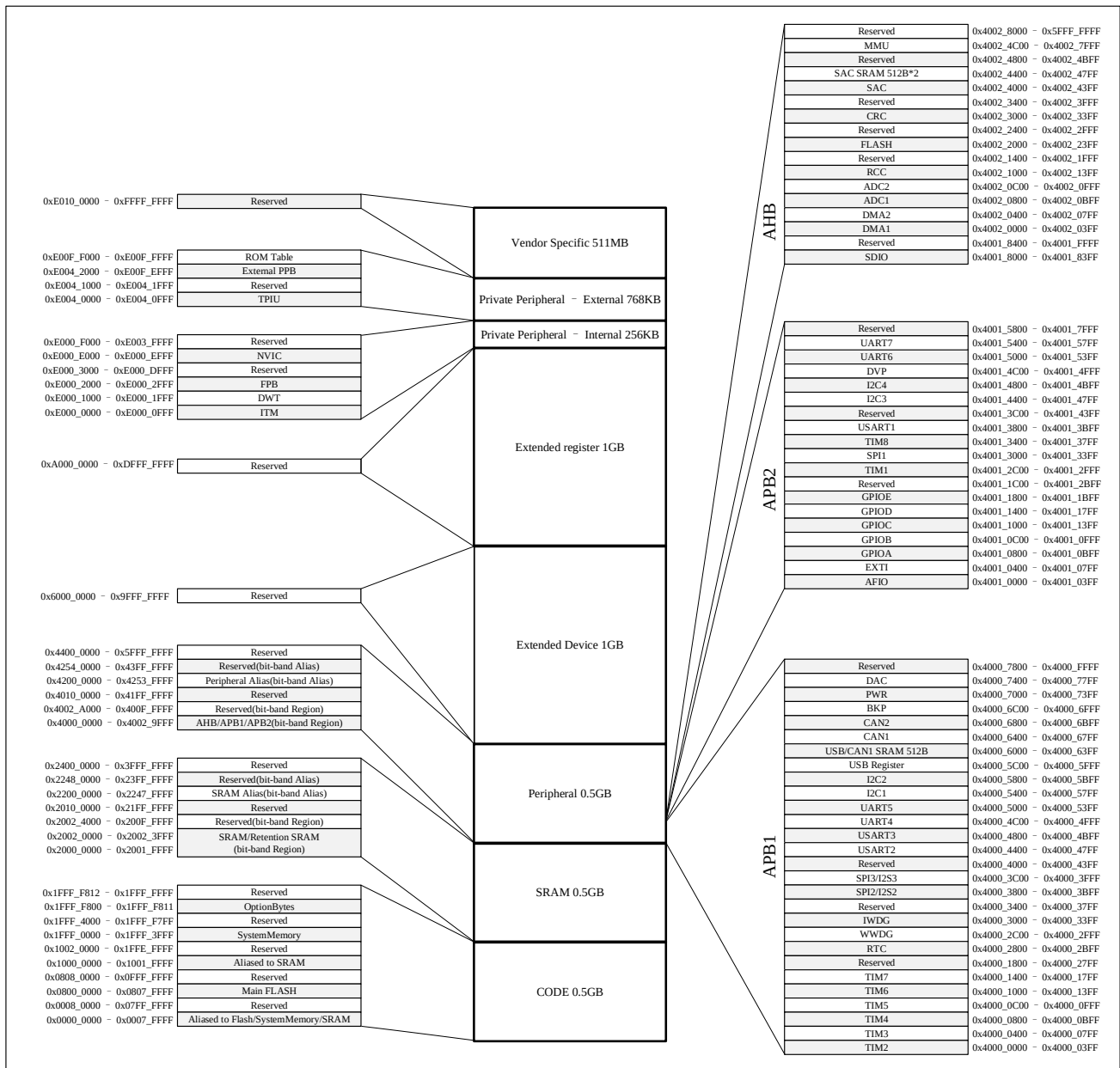
Figure 2-3 Bus address map
