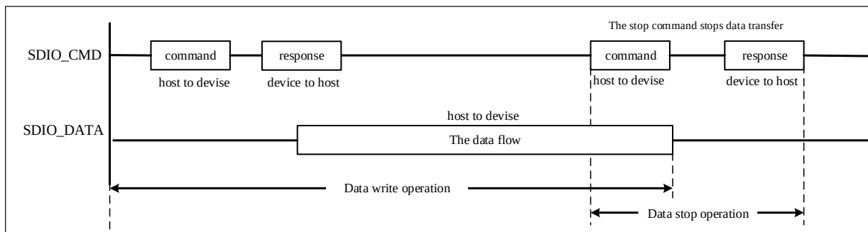
Figure 19-5 SDIO continuous write operation
