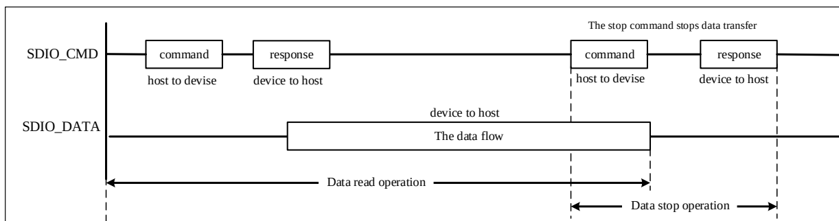
Figure 19-4 SDIO continuous read operation
