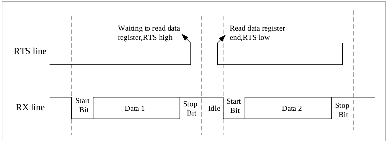
Figure 24-11 RTS flow control
