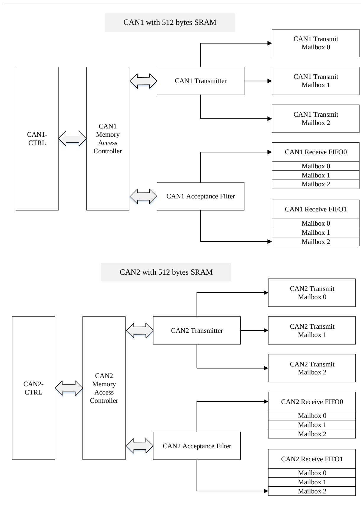
Figure 21-3 Dual CAN block diagram
