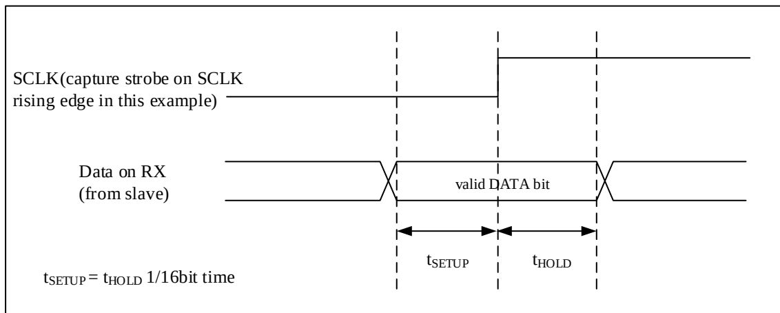
Figure 24-18 RX data sampling / holding time
