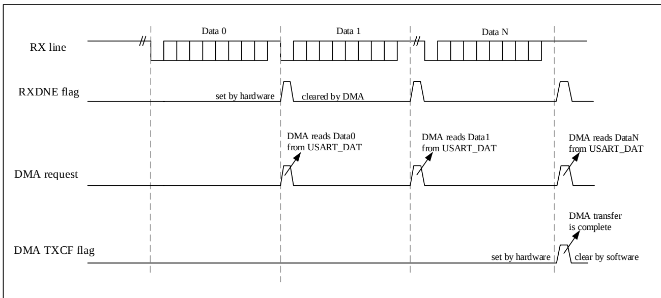
Figure 24-9 Reception using DMA
