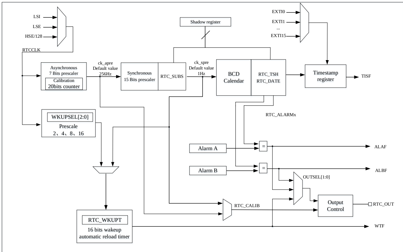
Figure 15-1 RTC Block Diagram
