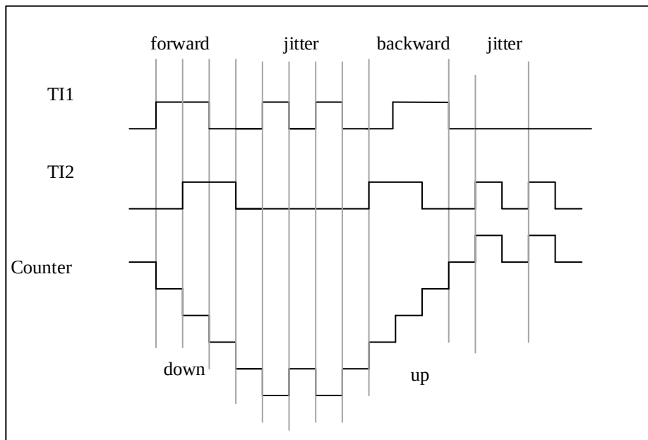
Figure 12-33 Encoder interface mode example with IC1FP1 polarity inverted
