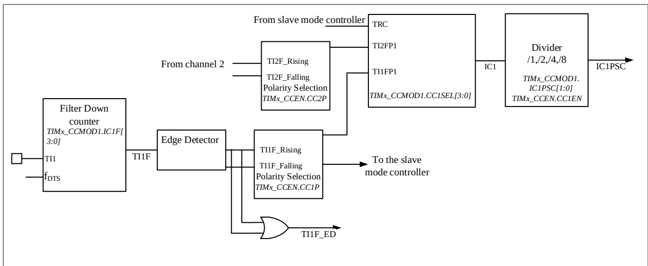
Figure 12-16 Capture/compare channel (example: channel 1 input stage)
