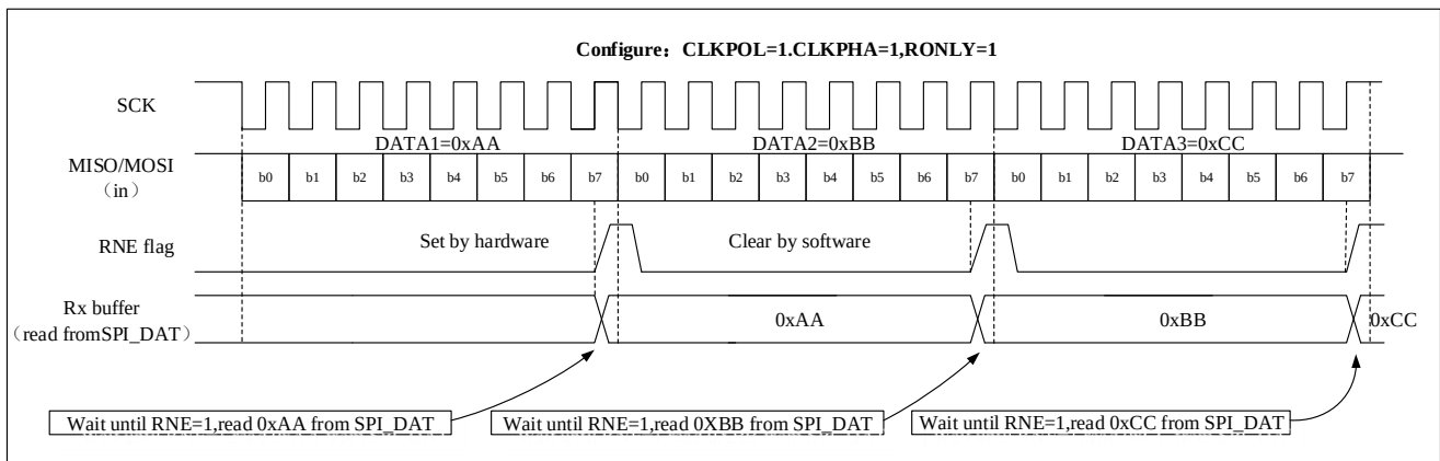
Figure 22-7 Schematic diagram of RNE change when continuous transmission occurs in receive-only mode (BIDIRMODE = 0 and RONLY = 1)
