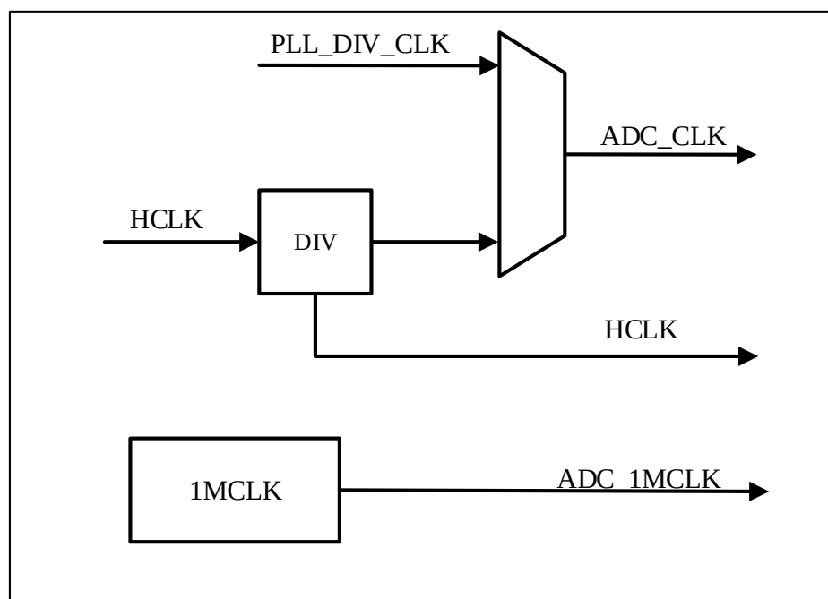
Figure 10-2 ADC clock
