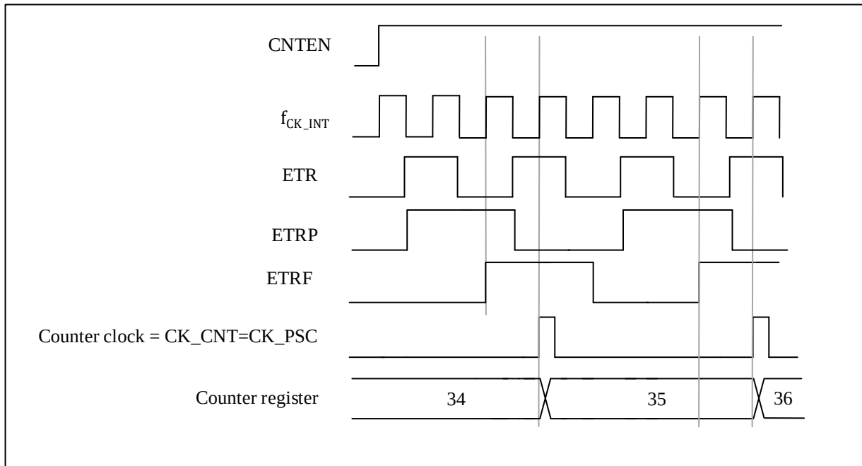
Figure 12-15 Control circuit in external clock mode 2
