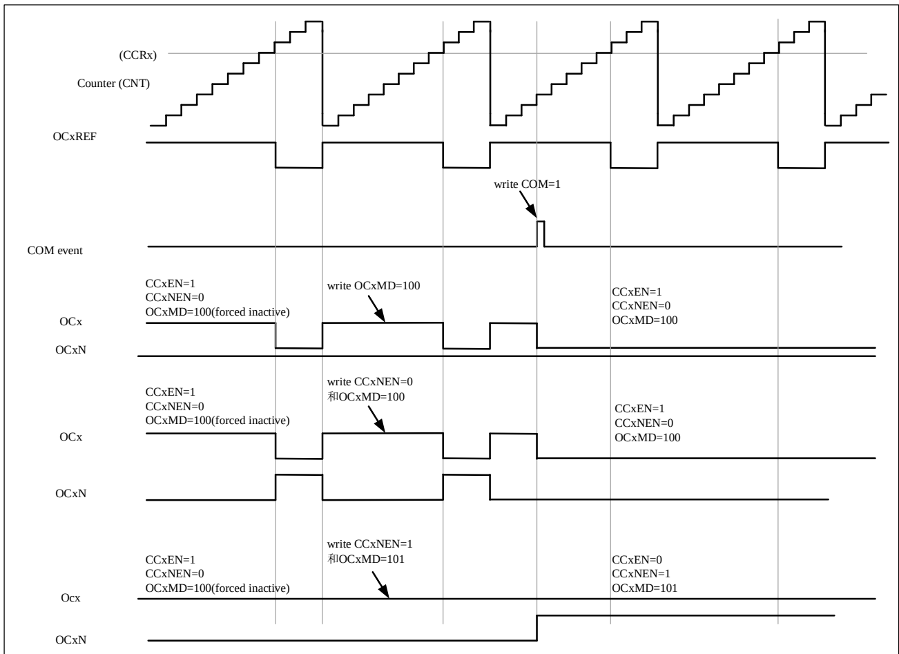
Figure 12-31 6-step PWM generation, COM example (OSSR=1)
