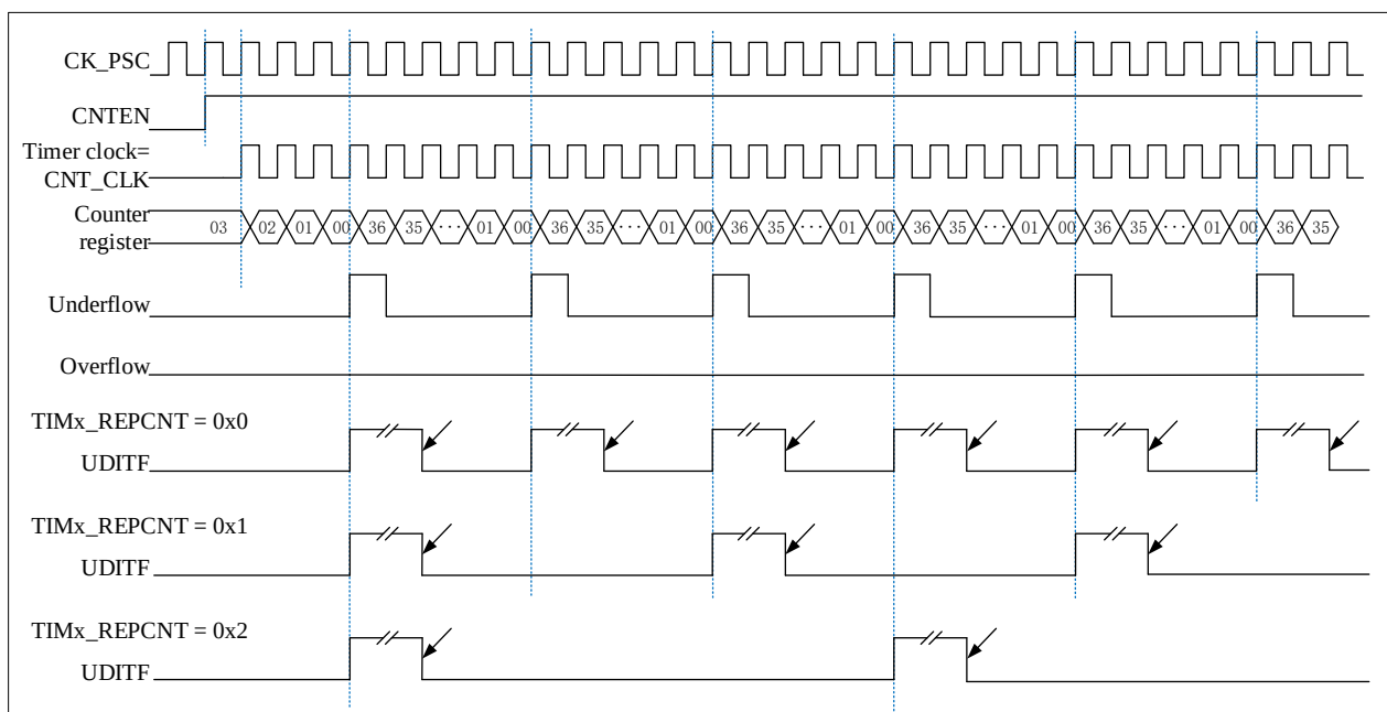
Figure 12-8 Repeat count sequence diagram in down-counting mode
