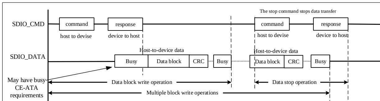
Figure 19-3 SDIO (multiple) data block write operation
