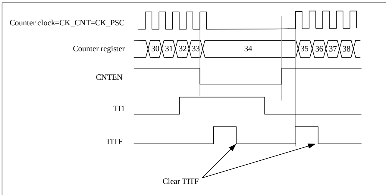
Figure 12-29 Control circuit in Gated mode
