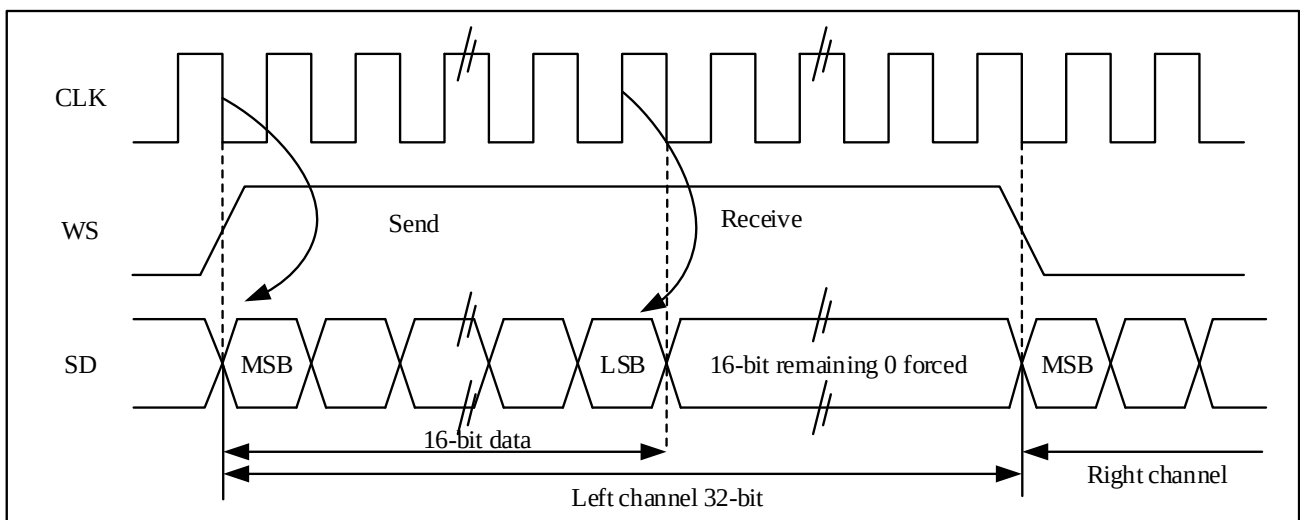
Figure 22-19 MSB-aligned 16-bit data is extended to 32-bit packet frame, CLKPOL = 0
