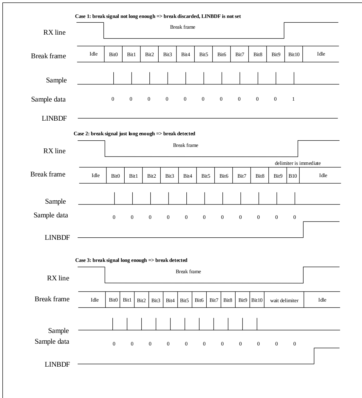
Figure 24-21 Break detection in LIN mode (11-bit break length-the LINBDL bit is set)
