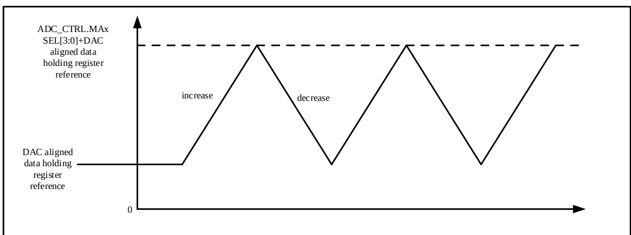
Figure 11-7 Triangle wave generation of DAC
