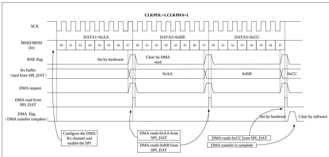
Figure 24-12 Reception using DMA
