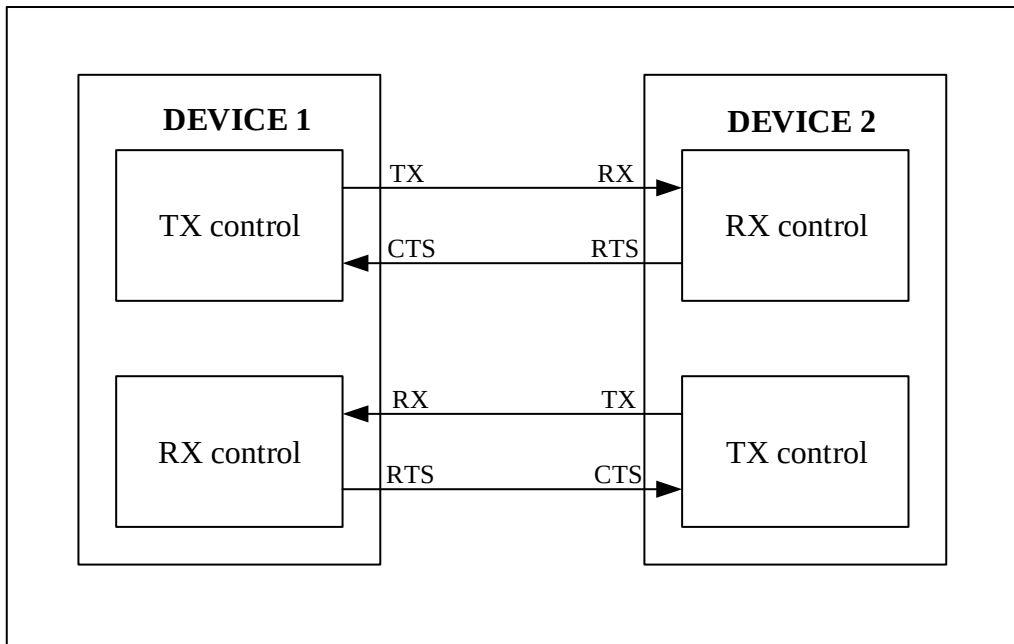
Figure 22-10 Hardware flow control between two USART
