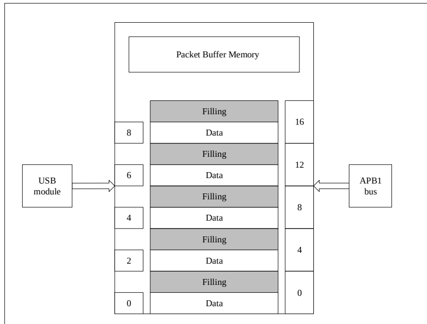
Figure 26-2 The user applications on the microcontrollers and the USB modules access Packet Buffer Memory
