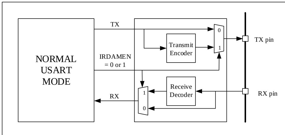
Figure 22-20 IrDA data Modulation (3/16)-normal mode
