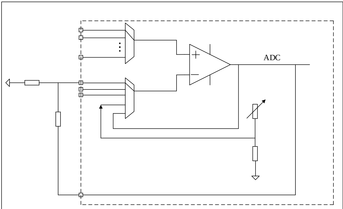
Figure 20-2 Independent op amp mode of OPAMP
