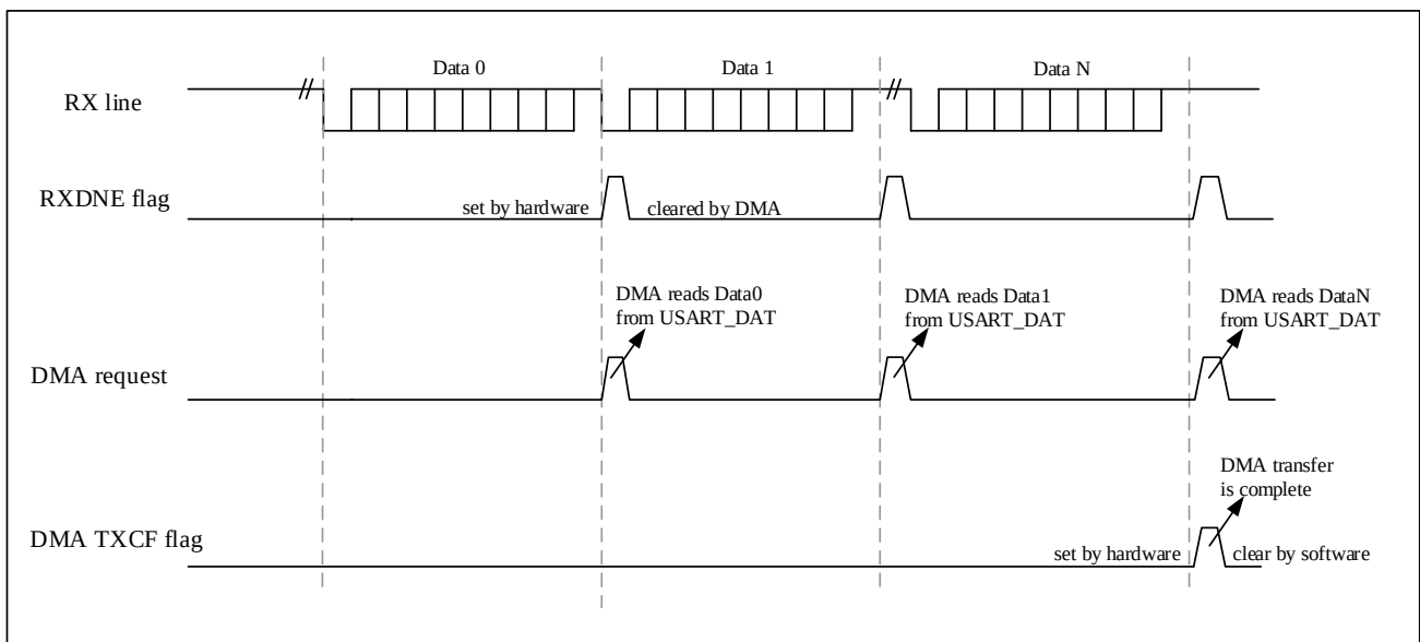
Figure 22-9 Reception using DMA
