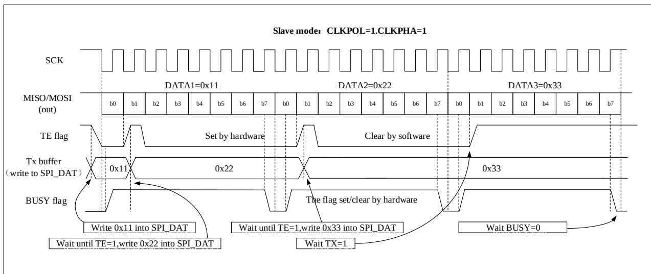
Figure 24-9 Schematic diagram of TE/BUSY change during continuous transmission in slave unidirectional transmit-only mode
