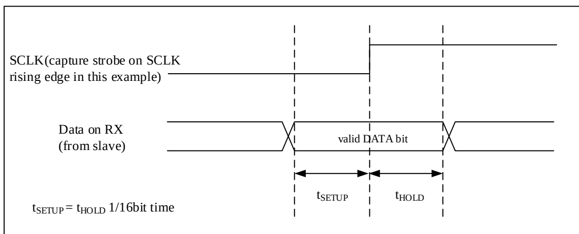
Figure 22-18 RX data sampling / holding time
