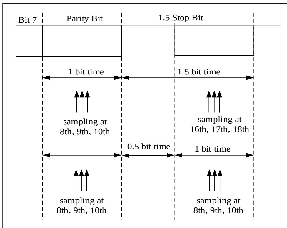
Figure 22-24 Use 1.5 stop bits to detect parity errors
