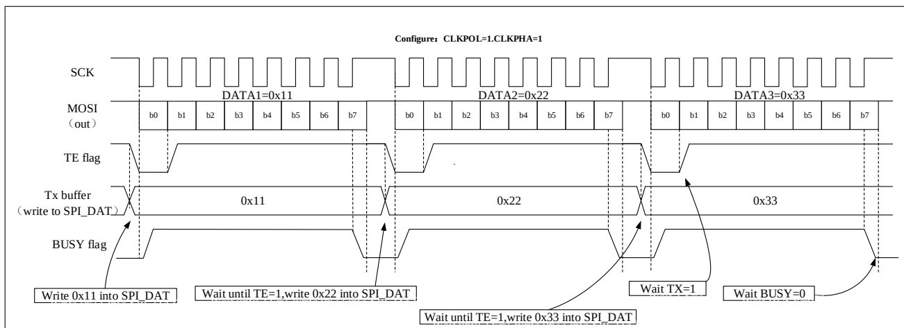
Figure 24-10 Schematic diagram of TE/BUSY change when BIDIRMODE = 0 and RONLY = 0 are transmitted discontinuously
