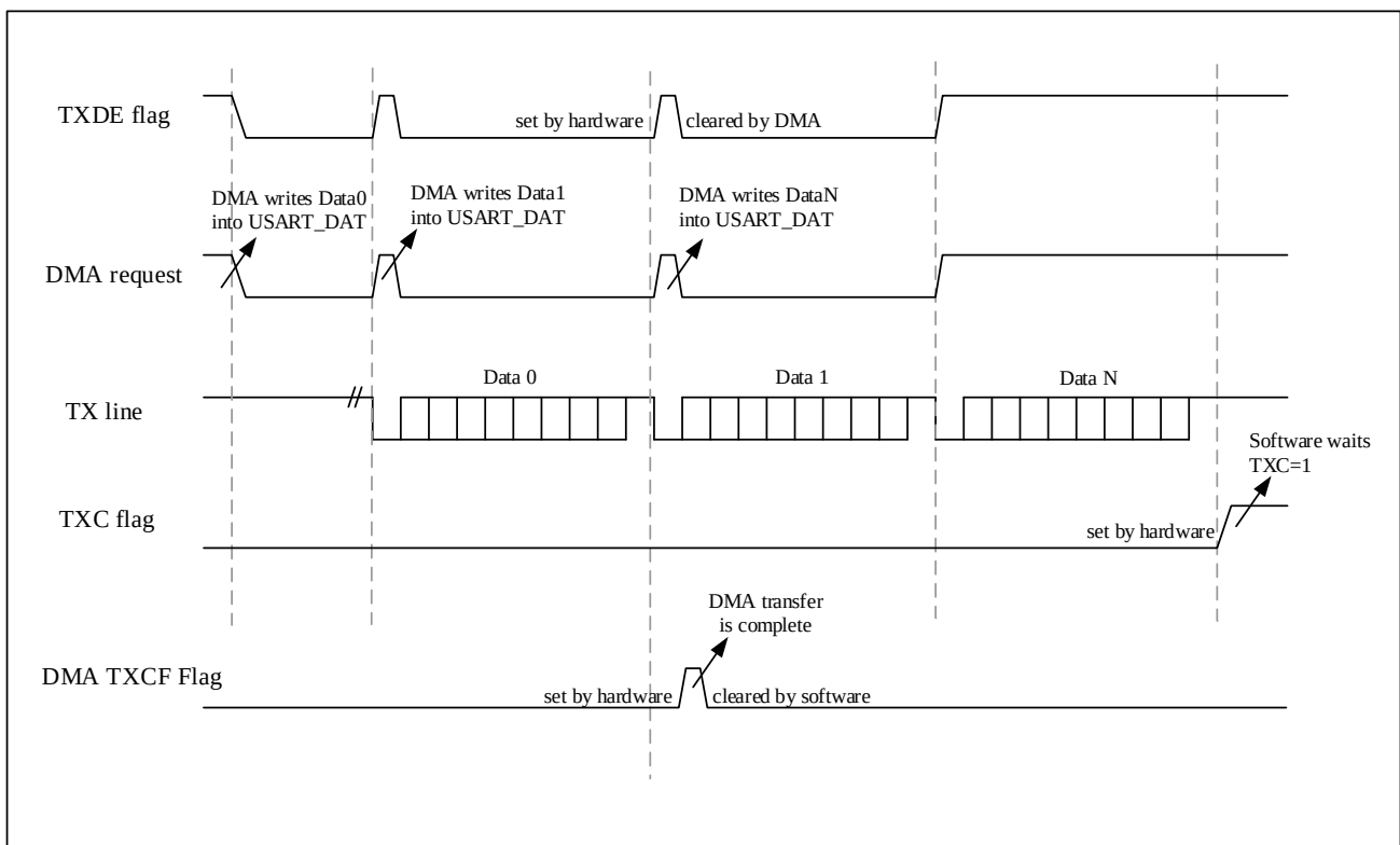
Figure 22-8 Transmission using DMA
