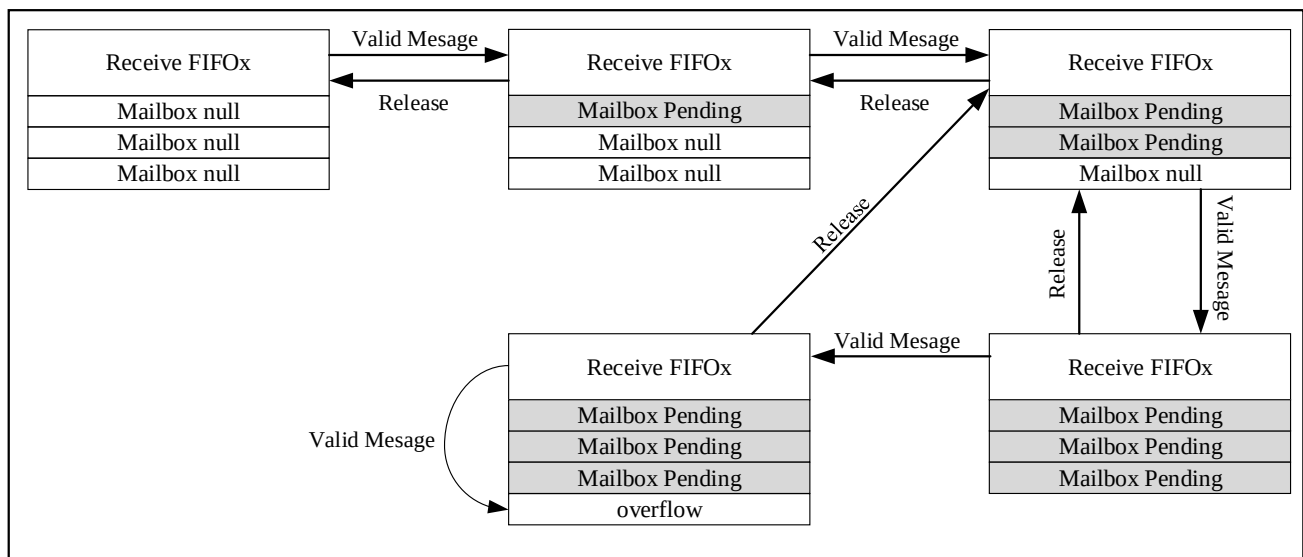
Figure 25-8 Receive FIFO status
