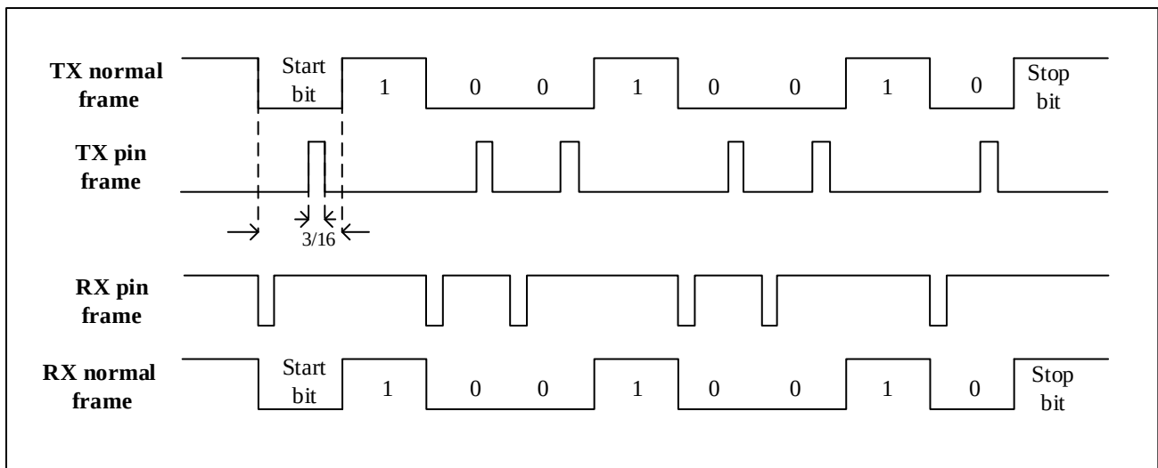
Figure 22-20 IrDA data Modulation (3/16)-normal mode
