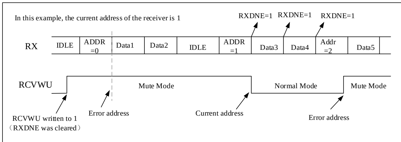
Figure 22-14 Mute mode detected using address mark
