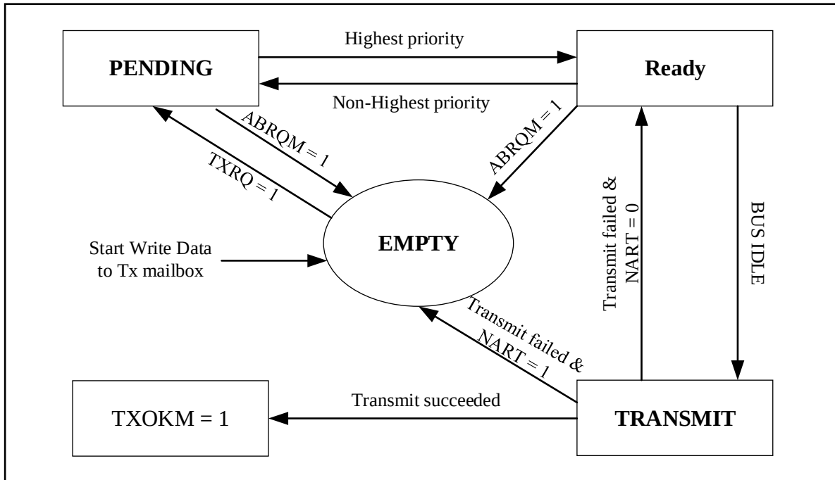
Figure 25-7 Send mailbox status
