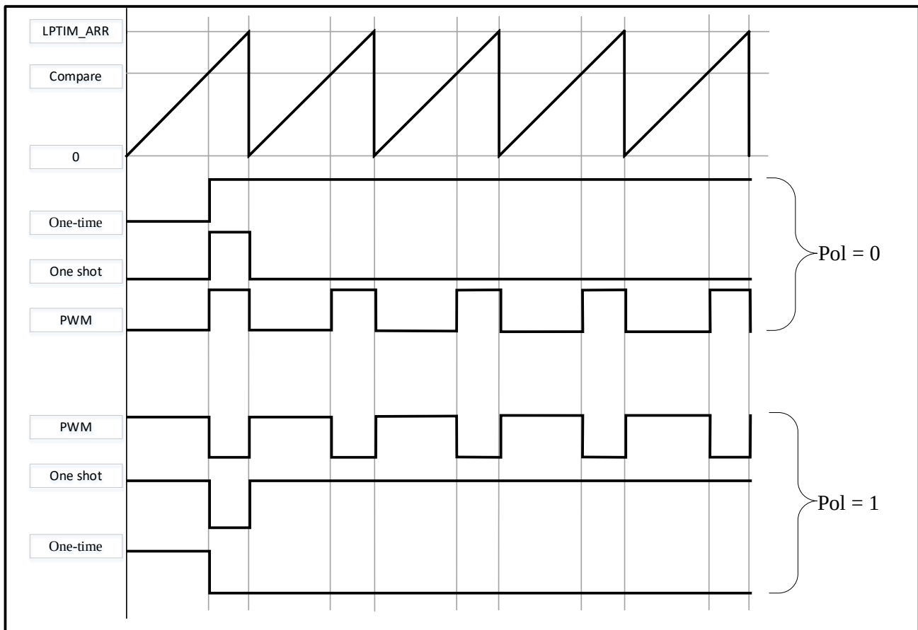
Figure 13-6 Waveform generation
