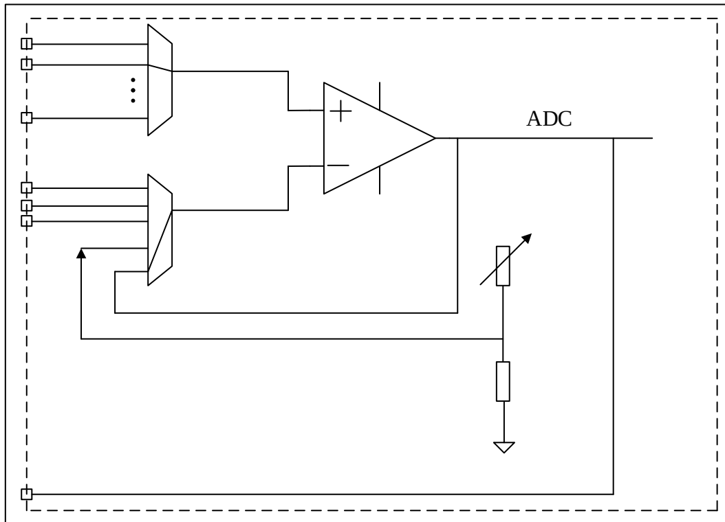
Figure 20-3 Follow mode
