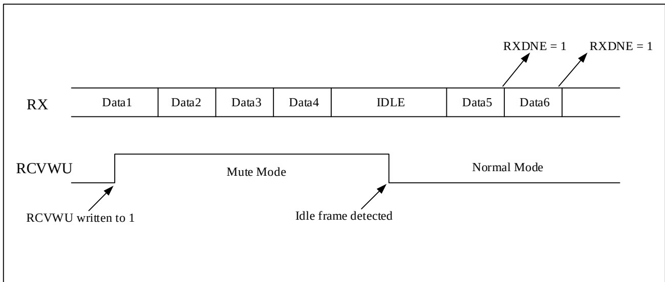
Figure 22-13 Mute mode using idle line detection
