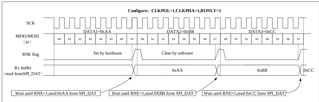
Figure 24-7 Schematic diagram of RNE change when continuous transmission occurs in receive-only mode (BIDIRMODE=0 and RONLY=1)
