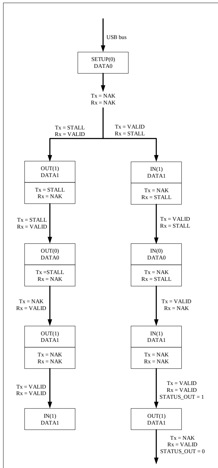
Figure 26-5 Control transfer
