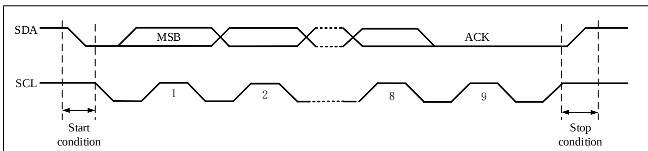
Figure 21-2 I 2 C bus protocol
