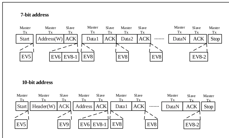
Figure 21-5 Master transmitter transfer sequence diagram
