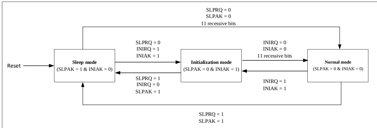
Figure 25-2 CAN working mode
