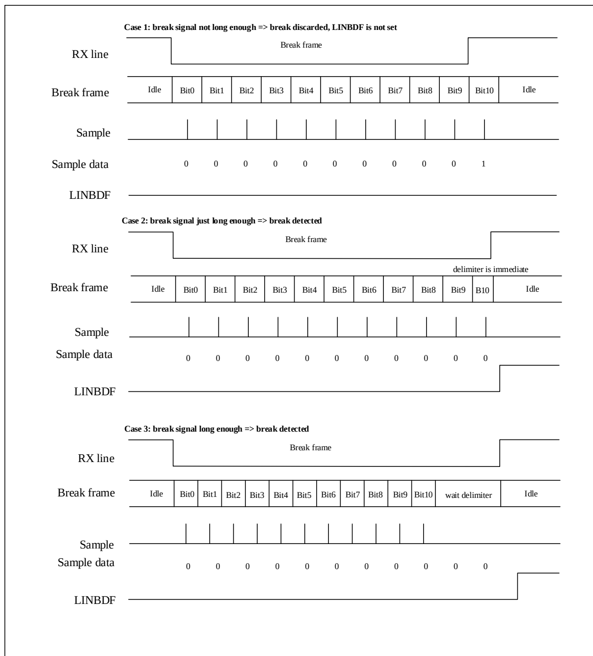
Figure 22-21 Break detection in LIN mode (11-bit break length-the LINBDL bit is set)
