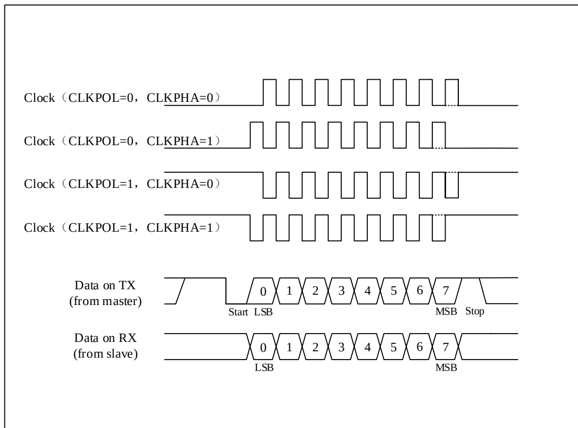
Figure 22-16 USART data clock timing example (WL=0)
