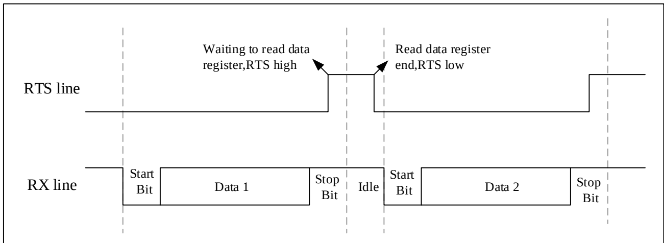
Figure 22-11 RTS flow control
