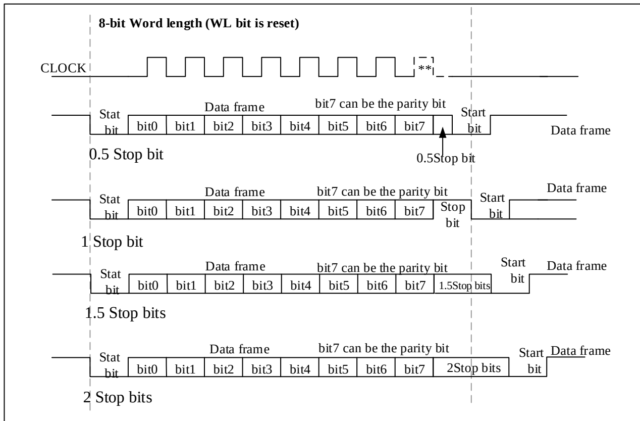
Figure 22-4 Configuration stop bit
