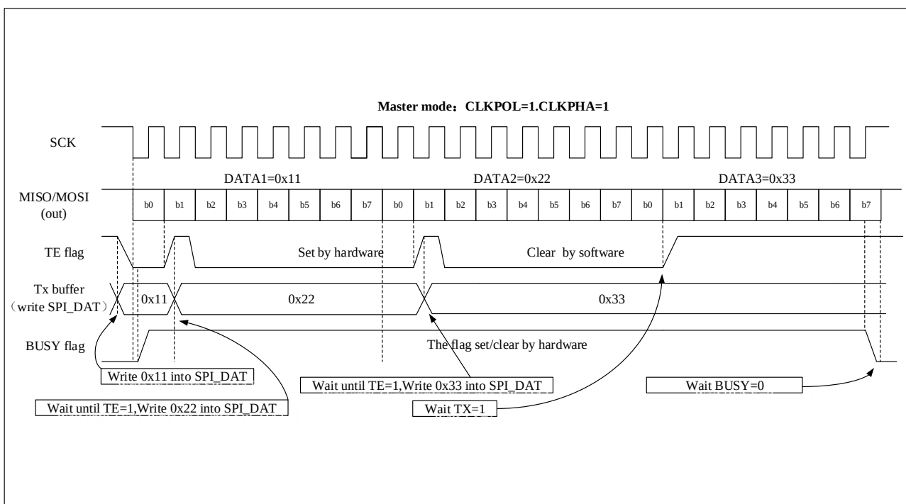
Figure 24-6 Schematic diagram of TE/BUSY change when host transmits continuously in one-way only mode
