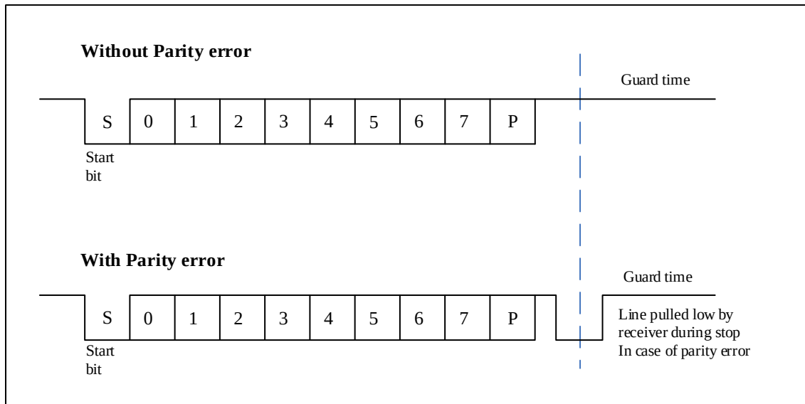
Figure 22-23 ISO7816-3 Asynchronous Protocol
