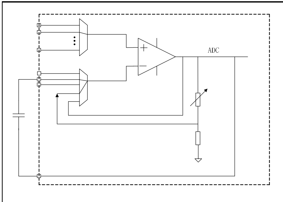
Figure 20-5 Internal gain mode with filter
