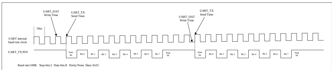
Figure 22-5 Transmit timing difference
