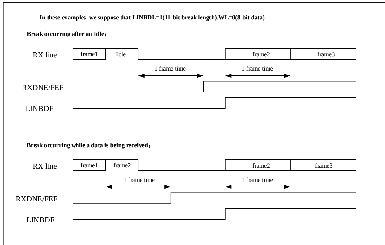
Figure 22-22 Break detection and framing error detection in LIN mode
