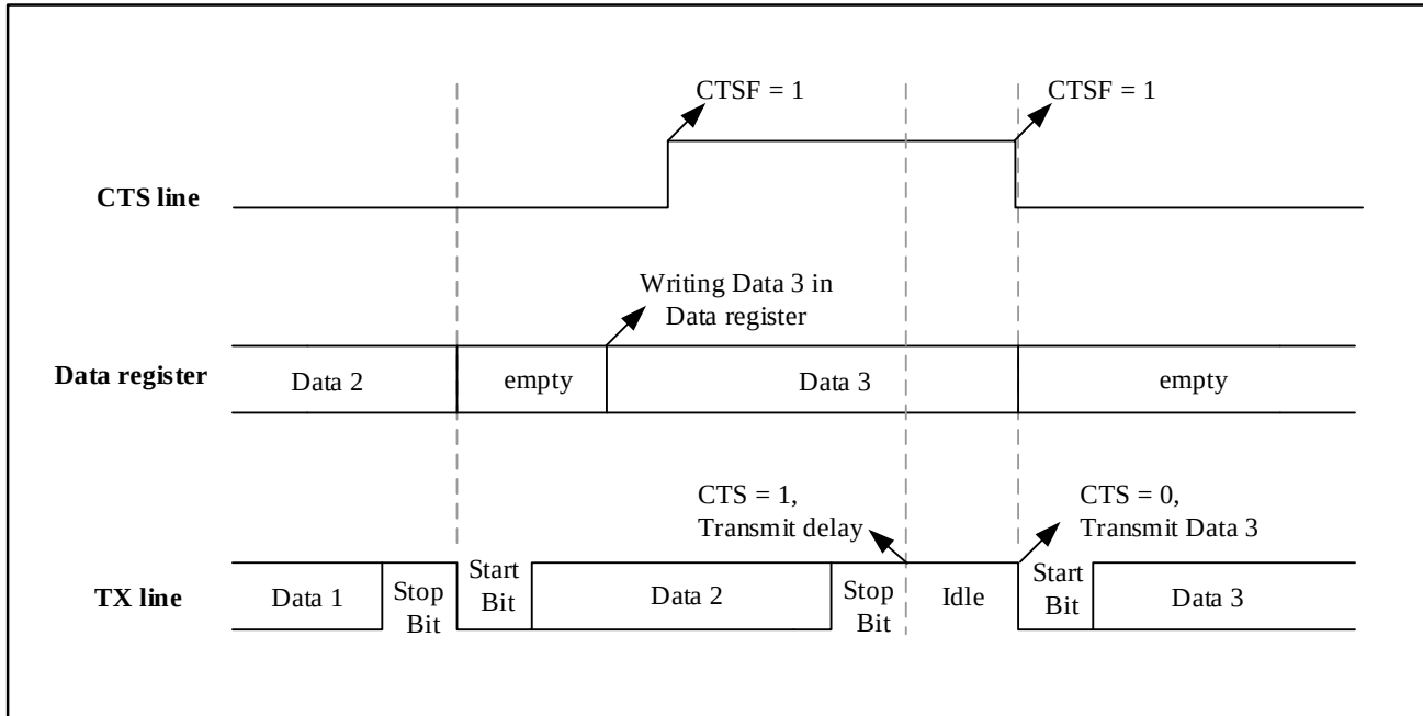
Figure 22-12 CTS flow controls
