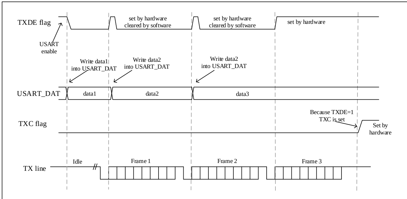
Figure 22-6 TXC/TXDE changes during transmission
