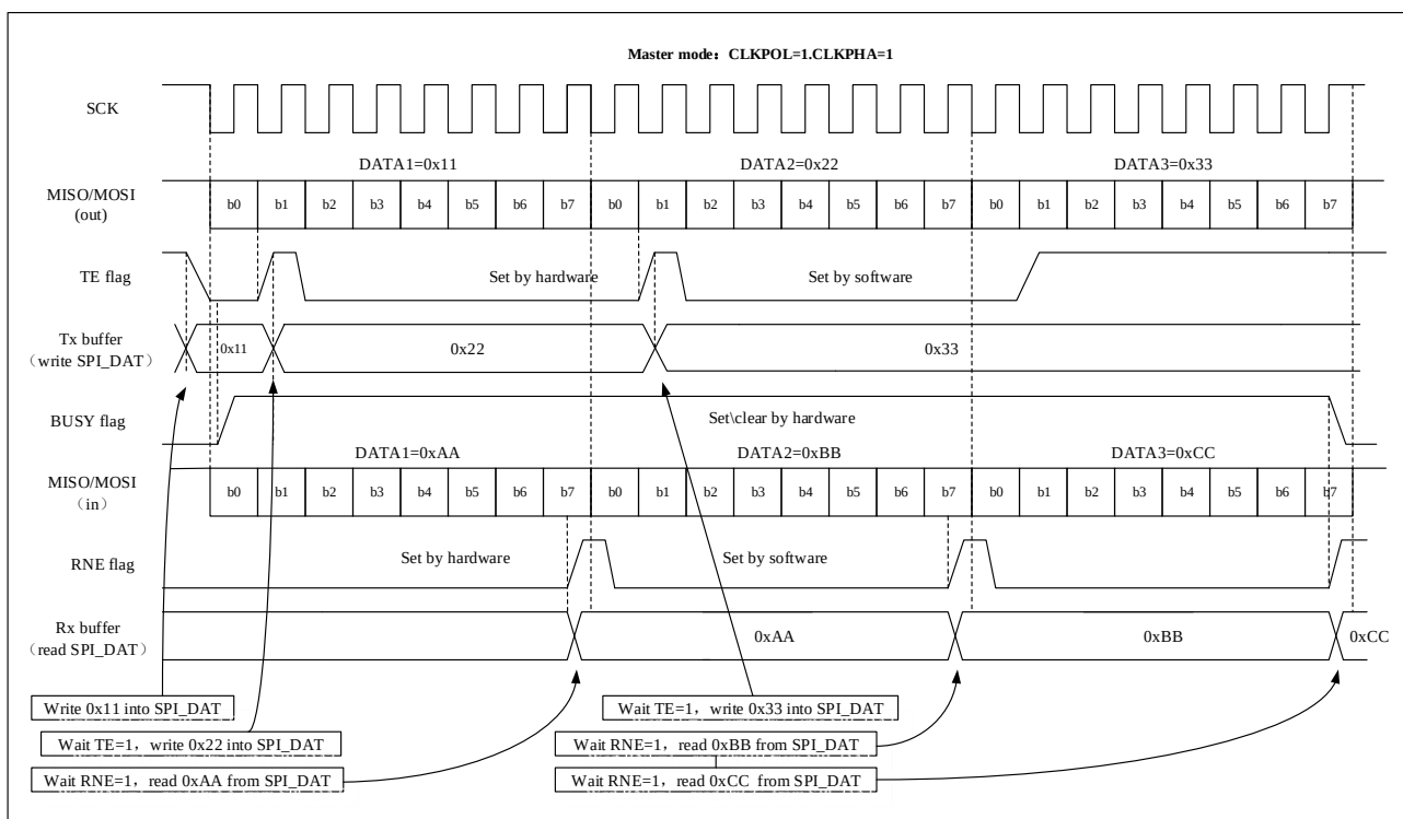
Figure 24-5 Schematic diagram of the change of TE/RNE/BUSY when the host is continuously transmitting in full duplex mode
